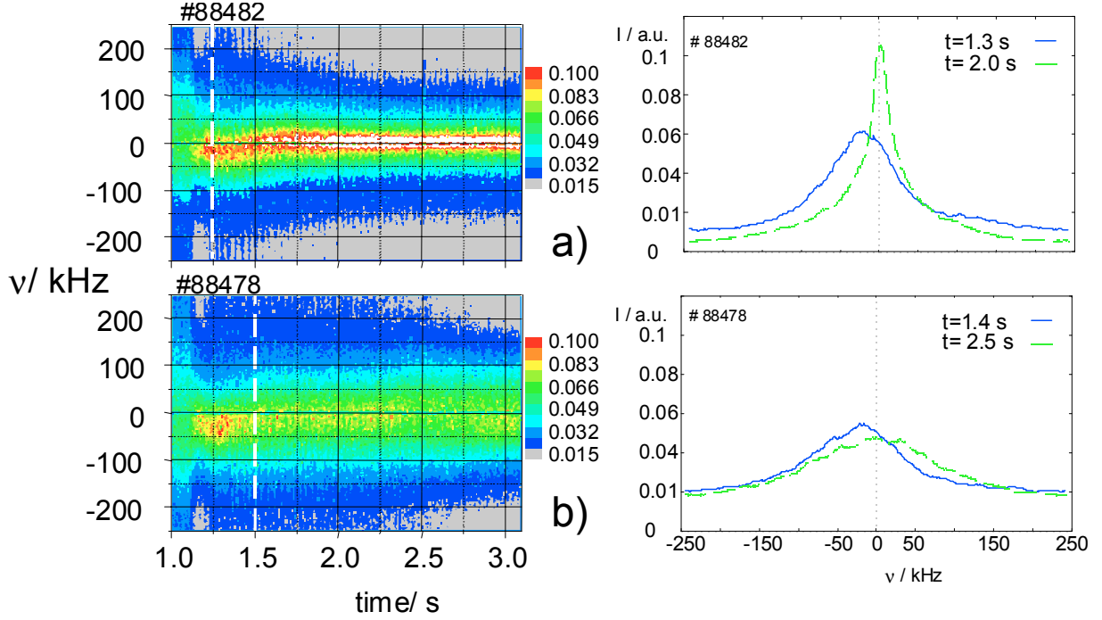
Fig 4 Time evolution of the amplitude spectra of density fluctuations measured by reflectometry (measured at the top of the machine about 2 cm inside the LCFS, cut-off density, n_{cut} = 1.7 \times 10^{19} \text{ m}^{-3} , frequency resolution \Delta F = 1.95 \text{ kHz} , time window \Delta t = 10.24 \text{ ms} ) and the spectra at a time before (blue solid lines) and during (green dashed lines) the gas fuelling. The start of gas fuelling is indicated by vertical white lines in the time evolution, case a) discharge #88482 (strong fuelling), case b) discharge #88478 (moderate fuelling), cf. Fig 1 for discharge parameters
