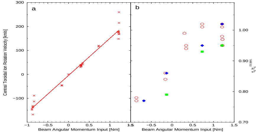
Figure 1: Angular Momentum Scan. a) The central toroidal rotation velocity of C^{6+} is shown versus the angular momentum input by means of Neutral Beams. The line is to guide the eye. b) shows the energy confinement time, normalized to the ITER89L scaling law, versus the angular momentum input. The red circles feature a density n_e = 2 \cdot 10^{19} \text{ m}^{-3} and a field B_\phi = 2.25 \text{ T} , the blue diamonds have n_e = 2 \cdot 10^{19} \text{ m}^{-3} and B_\phi = 2.5 \text{ T} , and the green rectangles have n_e = 3 \cdot 10^{19} \text{ m}^{-3} and B_\phi = 2.5 \text{ T} .
