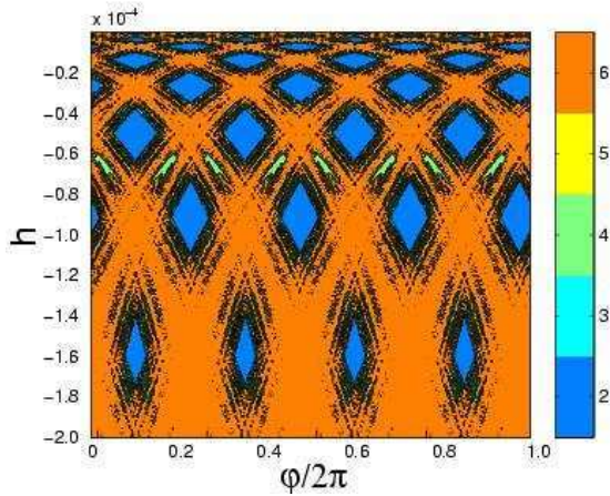
Figure 3: Laminar plot of field lines in the (\phi, \xi) plane ( h < 0 ) of the section \Sigma_s .
