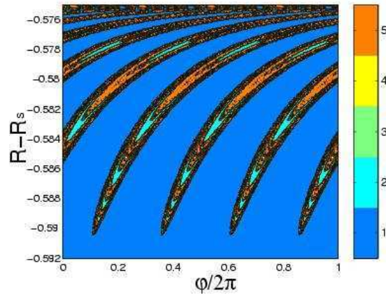
Figure 4: Magnetic footprint structure on the divertor plate in the (\phi, R) plane.
