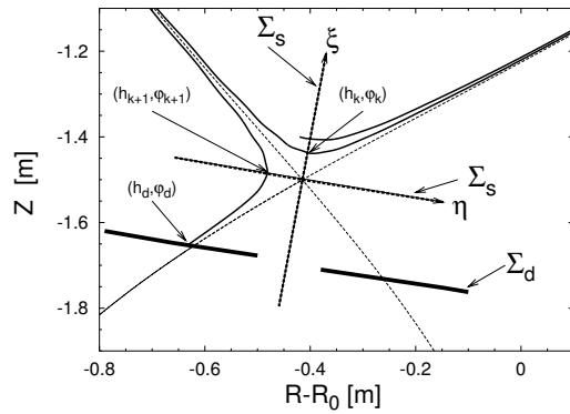
Figure 1: Scheme of mapping of field lines to the section \Sigma_s and to the divertor plates.
