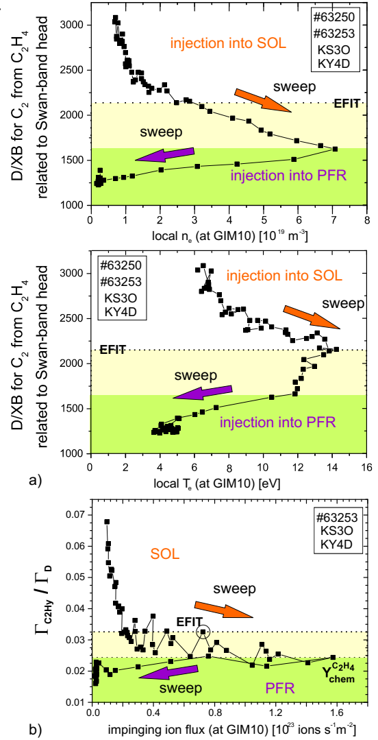
Figure 4: a) D/XB for C 2 from C 2 H 4 .
