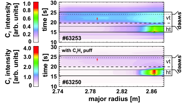
Figure 5: Radial distribution of the C 2 photon flux in the outer divertor measured with KT3.
