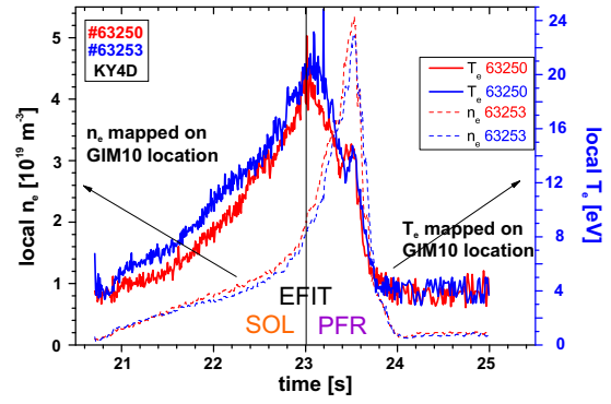
Figure 2: Local T_e and n_e profiles.
