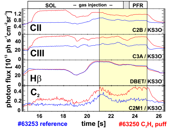
Figure 3: Photon flux time evolution.
