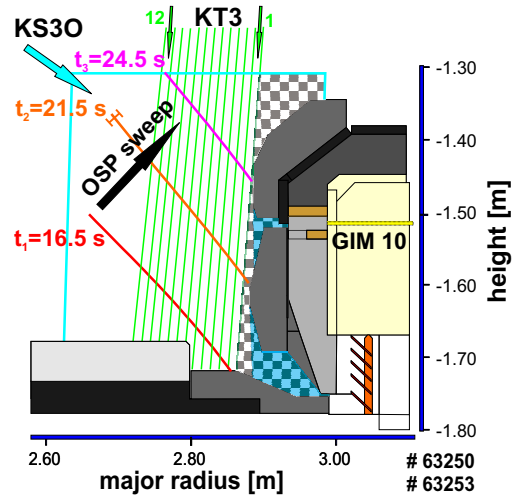
Figure 1: Outer divertor: strike-point sweep and spectroscopic systems.
