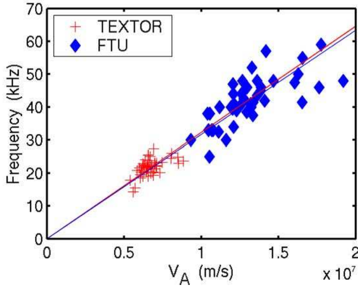
Figure 3. HF modes frequency versus Alfvén velocity calculated with line-average density. Solid red line: slope from a linear fit to TEXTOR data only. Blue line: same for FTU.
