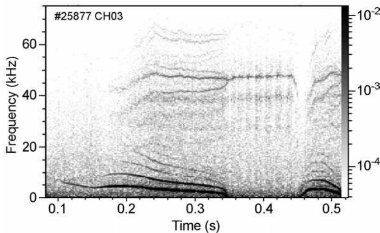
Figure 1. Spectrogram of a Mirnov coil signal in an ohmic FTU pulse. Greyscale gives the relative amplitude of poloidal field oscillations \delta B_{pol}/B_{pol} . Lines below 20 kHz correspond to a (-2, -1) tearing mode. The intense HF line near 50 kHz has n=-1 , the other just below has n=1 .
