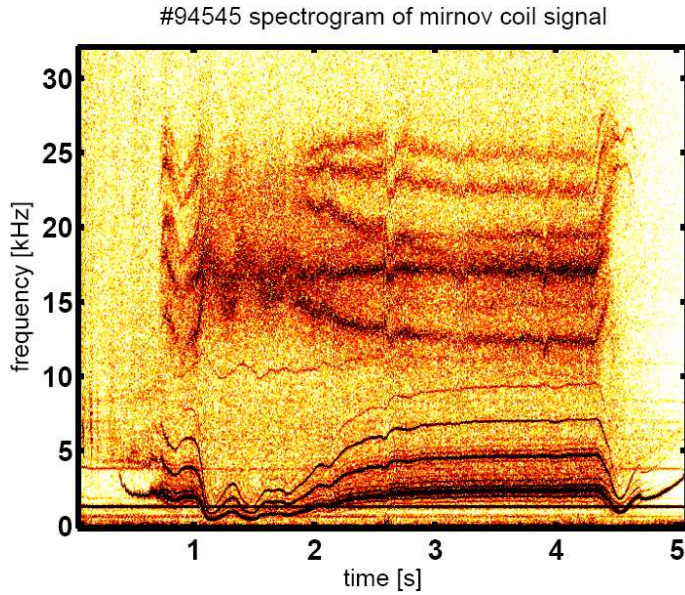
Figure 2. Spectrogram of a Mirnov coil signal in an ohmic TEXTOR pulse. Lines below 10 kHz correspond to a (-2, -1) tearing mode and its harmonics. The HF-modes higher than 12 kHz have alternating positive and negative mode numbers.
