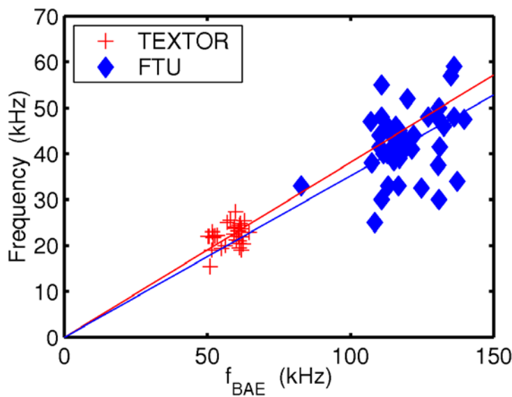
Figure 4. HF modes frequency versus BAE frequency accumulation point calculated with central temperature and T_e = T_i . Solid red line: slope from a fit to TEXTOR data only. Blue line: same for FTU.
