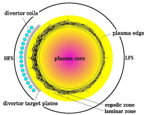
Fig. 1: Schematic representation of the DED coils and the main plasma regions. (Adapted from [5]).
