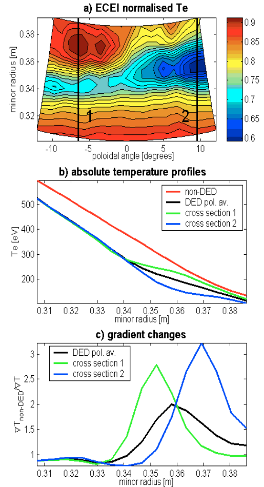
Fig. 4: Comparison of T_e profiles during DED with non-DED reference.
