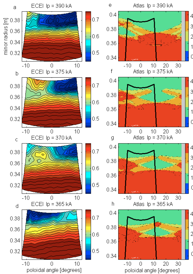
Fig 3 Comparison of ECEI temperature measurements with Atlas calculations of the connection length (laminar plots) during a plasma current ramp.
