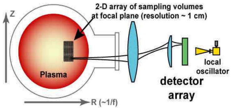
Fig. 2: Schematic representation of the ECE-Imaging system.
