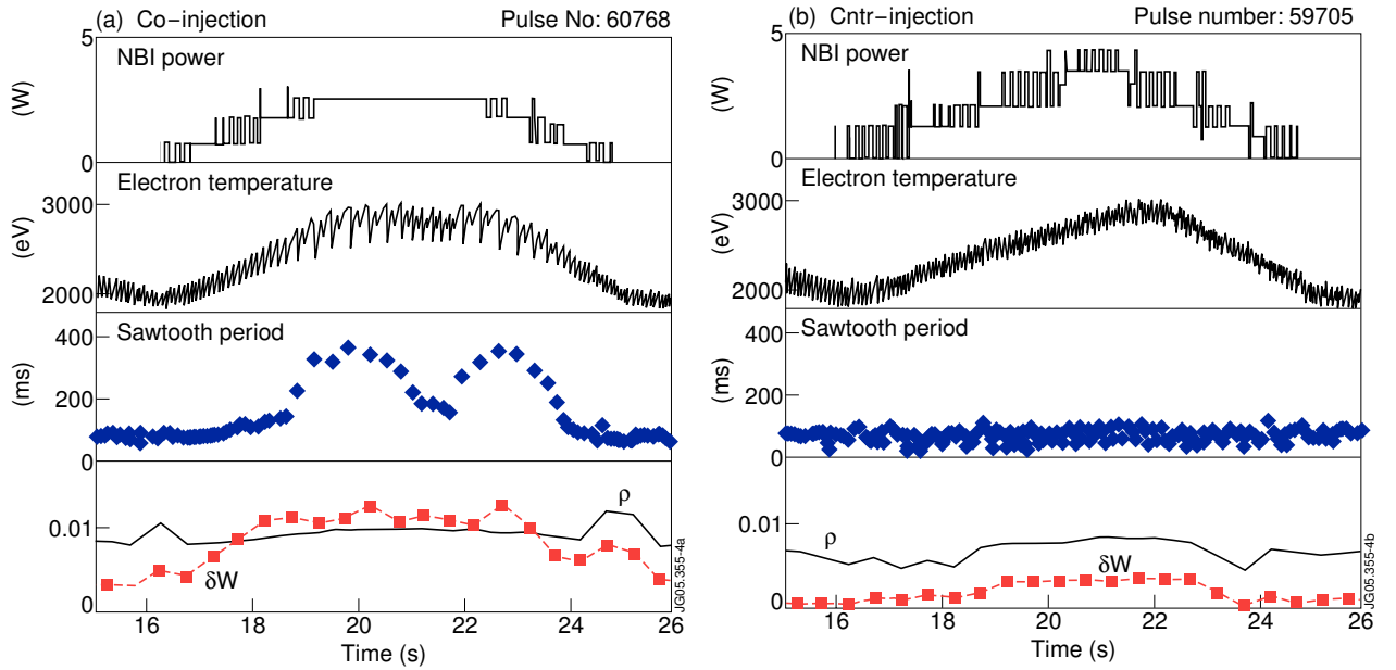
Figure 4: Showing two otherwise similar NBI ramping discharges with opposite NBI orientation [16]. Also compared are the expressions \delta W = \pi \delta \hat{W}/s_l and \rho = c_r \rho_i in the macroscopic threshold instability criterion of Eq.2.
