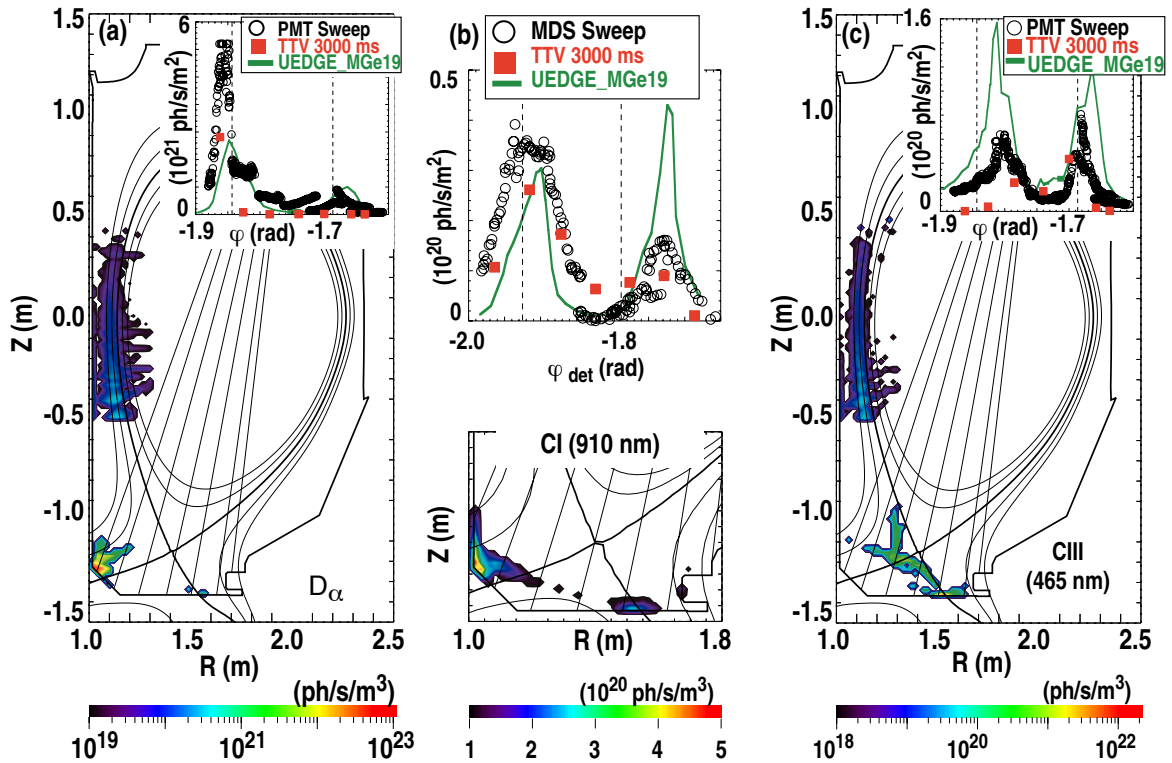
Fig. 2. Reconstructed D_\alpha (a), CI (910 nm, b), and CIII (465 nm, c) intensity distribution from image data of the lower and high field, midplane SOL. The inserts show the poloidal profile of the emissions at the same wavelength obtained by the vertically viewing PMT and spectrometer arrays during the strike point sweep, compared to the same line-integrals across the reconstructed images, and the UEDGE/DEGAS2 plasmas solution. In the inserts the dashed lines indicate the location of the separatrix at the inner and outer target.
