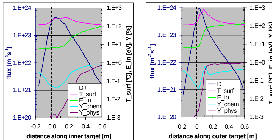
Figure 2 Profiles of deuterium ion flux, surface temperature, impact energy, chemical erosion and physical sputtering yield along the divertor plates (left – inner, right – outer divertor).
