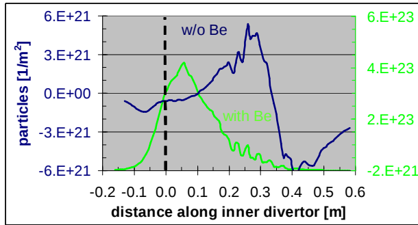
Figure 4 Profile of net-carbon erosion/deposition after 10s and same profile but with beryllium deposition added.
