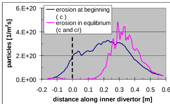
Figure 3a Erosion profile along inner divertor plates of graphite (c) at the beginning and of graphite plus redeposited carbon (c+cr) in equilibrium.
