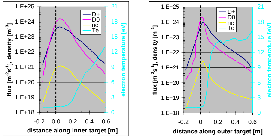
Figure 1 Deuterium ion and atom flux, electron density and temperature along inner (left) and outer (right) divertor target plate (from B2-EIRENE).
