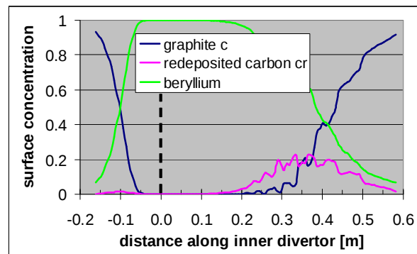
Figure 3b Surface concentration along inner divertor plates of graphite (c), redeposited carbon (cr) and beryllium (be) in equilibrium.
