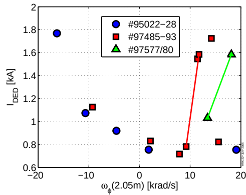
Figure 3: Plasma rotation scan using various NBI beam compositions.
