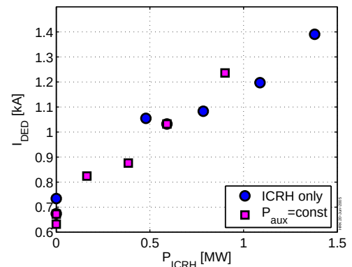
Figure 2: ICRH scans with and without constant beta.
