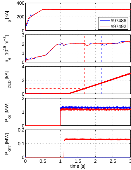
Figure 1: Time traces of two discharges with slightly different beam composition.
