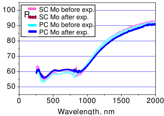
Fig.2. Total reflectivity of molybdenum mirrors before and after exposure
