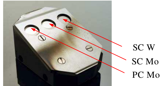
Fig. 1. The limiter with mirrors after exposure in the SOL of TEXTOR
