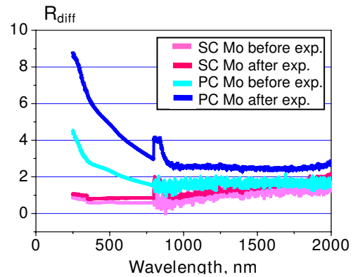
Fig. 3. Diffuse reflectivity of molybdenum mirrors before and after exposure
