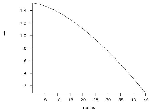
Figure 1: Ion temperature T_i [keV] (ALCA-TOR) versus radius r [cm].
