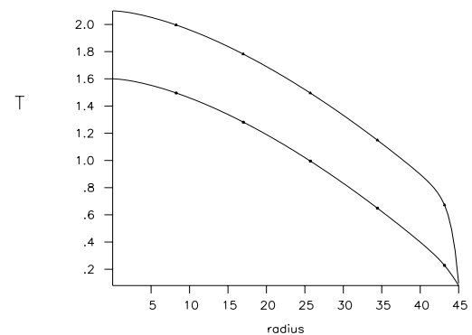
Figure 5: L- and H - mode temperatures in a medium size Tokamak versus radius r [cm].
