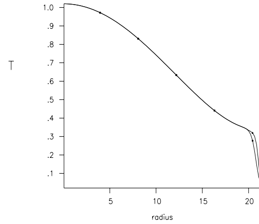
Figure 4: Computed (upper curve) and measured ion temperature in ALCATOR [keV]
