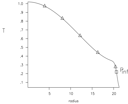
Figure 1: Ion temperature T_i [keV] (ALCA-TOR) versus radius r [cm].
