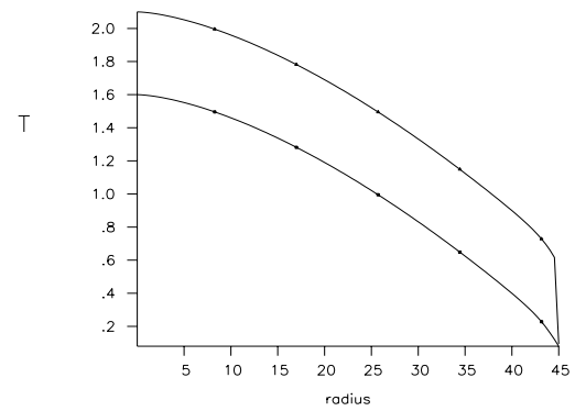
Figure 4: Computed (upper curve) and measured ion temperature in ALCATOR [keV]
