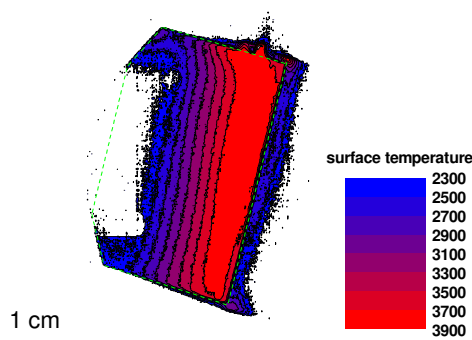
Fig.1 Surface temperature distribution on the tungsten plate.
