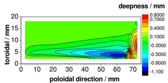
Fig.3 The surface profile in the molten zone.
