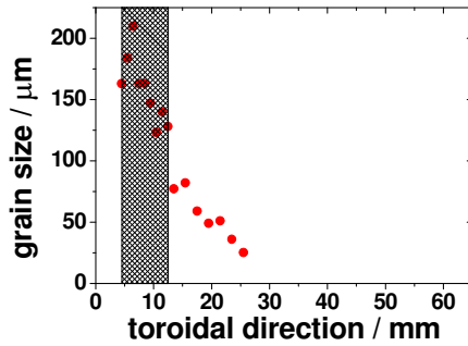
Fig.5 Dependence grain size on the position.
