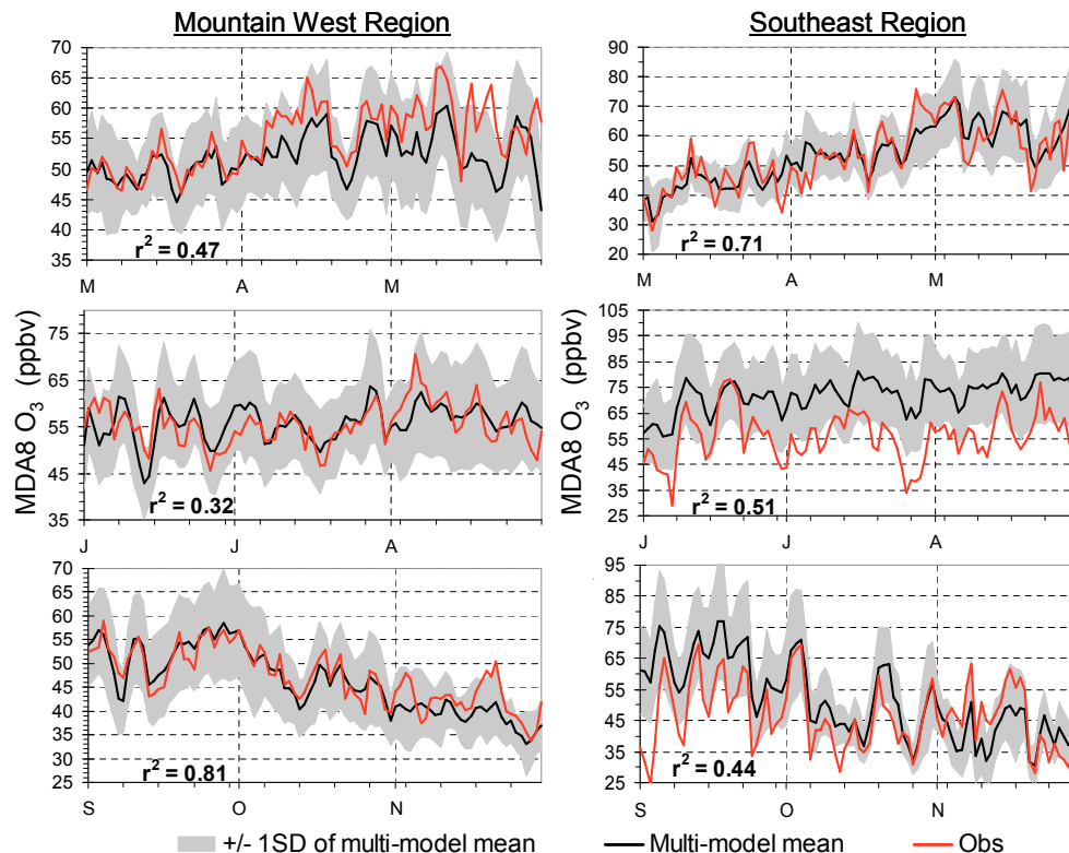
Fig. 5. Daily MDA8 O 3 from observations (red line), multi-model mean (black line) and 1 \sigma of the multi-model mean (gray shading) for spring (MAM), summer (JJA) and autumn (SON) in the Mountain West region (left) and Southeast region (right) depicted in Fig. 1. Note the range of magnitudes on the y-axes.
