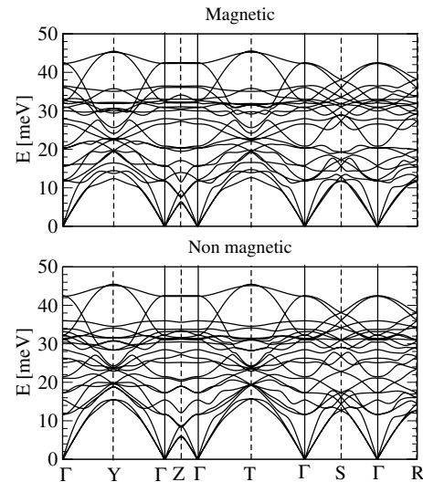
FIG. 5. Phonon dispersion relations for CaFeAsF from ab initio calculations. In the upper panel, magnetic refers to average magnetic calculations. The Bradley-Cracknell notation is used for the high-symmetry points along which the dispersion relations are obtained: Y=(12,1/2,0) , Z=(0,0,1/2) , T=(1/2,1/2,1/2) , S=(0,1/2,0) , and R=(0,1/2,1/2) .
