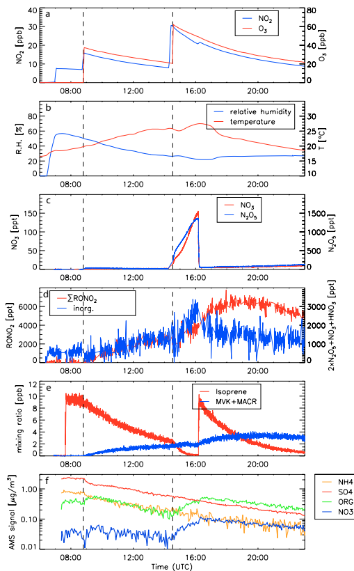
Fig. 1. Descending top to bottom, measurements of (a) \text{NO}_2 and \text{O}_3 (CL measurement), (b) chamber temperature and relative humidity (RH), (c) \text{NO}_3 and \text{N}_2\text{O}_5 (CaRDS), (d) organic nitrates ( \text{RONO}_2 ) and inorganic nitrates ( \text{NO}_3 + 2 \times \text{N}_2\text{O}_5 + \text{HNO}_3 ) (TD-LIF), (e) isoprene and the sum of methacrolein and methyl vinyl ketone (PTR-MS), and (f) AMS measurements of aerosol composition.
