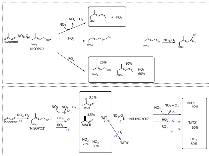
Fig. 2. Top: schematic of isoprene+ \text{NO}_3 mechanism MCM V3.1. 100% of first generation oxidation products are alkyl nitrates. The only first generation product which is reactive towards \text{NO}_3 is the carbonyl nitrate, which reacts in an aldehyde+ \text{NO}_3 mechanism at a rate of 1.1 \times 10^{-14} \text{ cm}^3 \text{ s}^{-1} . Bottom: the modified mechanism used in this study. NIT1–NIT4 are lumped species representing organic nitrates produced by the first (NIT1) and second (NIT2, NIT3, NIT4) oxidation steps. NIT1 has one \text{RONO}_2 group and one carbon-carbon double bond. Oxidation of the second double bond by \text{NO}_3 is presumed to either leave the original nitrate functionality (NIT2) or add an additional \text{RONO}_2 group (NIT3). Oxidation of NIT1 by \text{O}_3 is presumed to leave the nitrate functionality (NIT4). NIT1NO3OO is the peroxy radical generated by reaction of NIT1 with \text{NO}_3 followed by \text{O}_2 .
