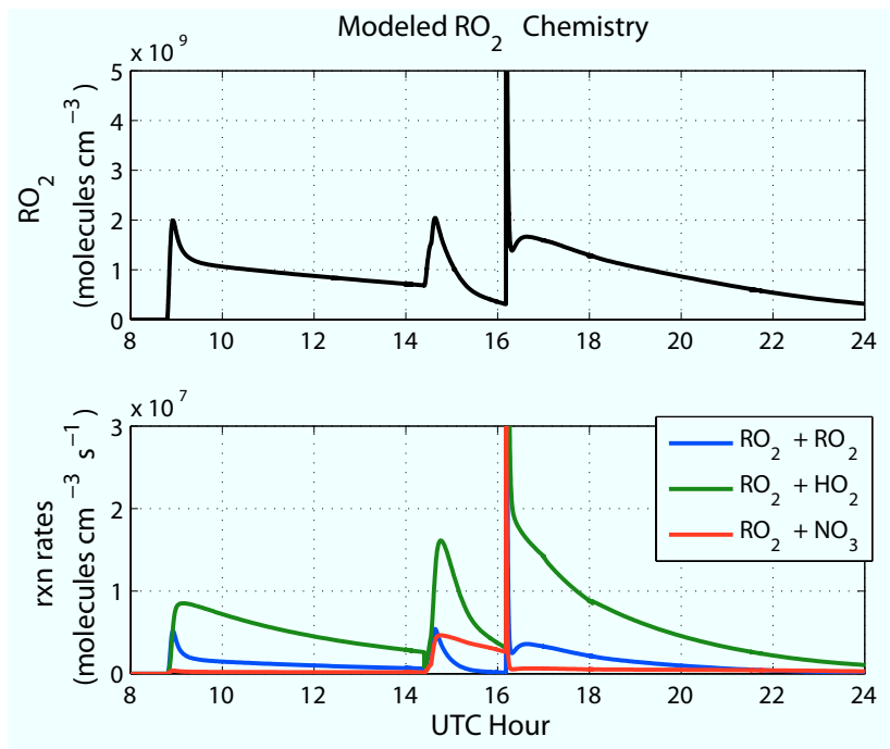
Fig. 6. Modeled calculations of (top) total peroxy radicals concentrations, and (bottom) sum of the rates of all \text{RO}_2 + \text{RO}_2 reactions (blue), all \text{RO}_2 + \text{HO}_2 reactions (green) and all \text{RO}_2 + \text{NO}_3 reactions (red).
