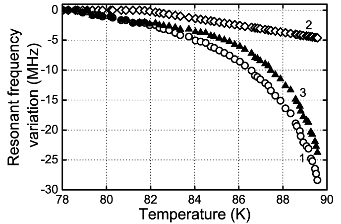
Fig. 3. Temperature dependence of resonance frequency variation for QDR with CEP: 1—Y-123; 2—Ti; 3—curve is difference of curves 1 and 2.
