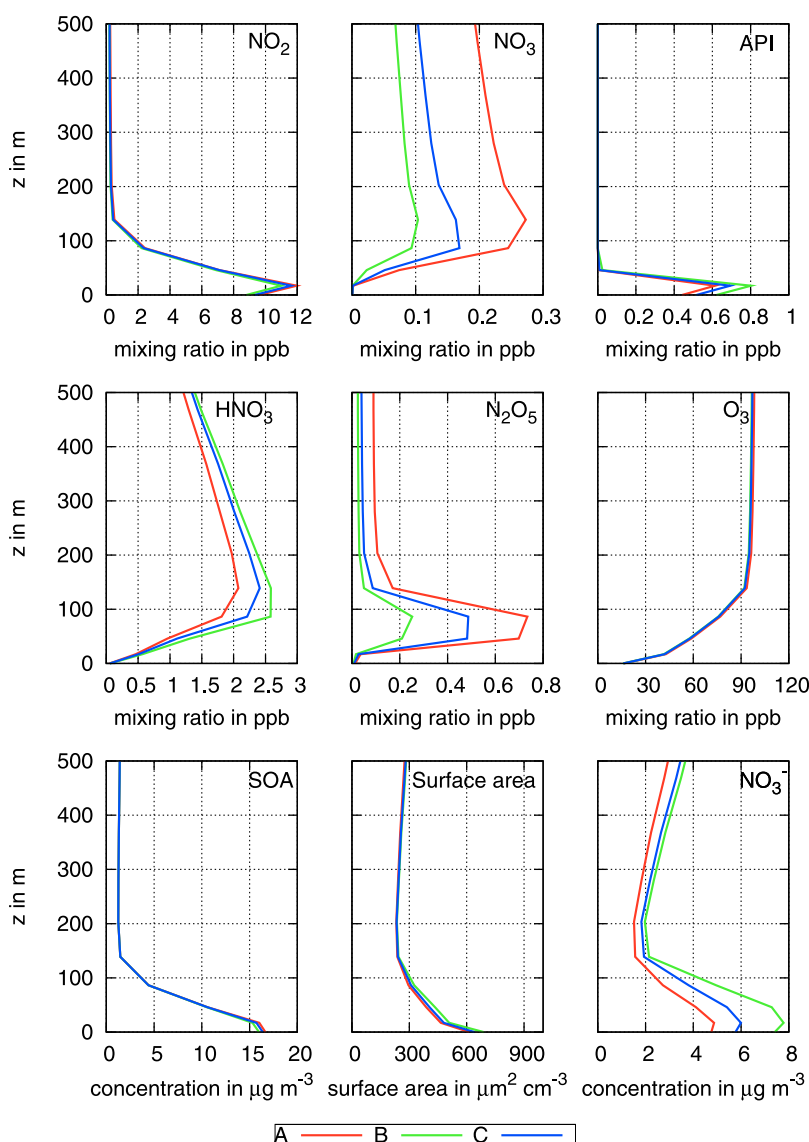
Figure 1. Simulated vertical profiles (at 0300 central European time, CET) of \text{NO}_2 , \text{NO}_3 , \alpha -pinene (API), \text{HNO}_3 , \text{N}_2\text{O}_5 , \text{O}_3 , SOA, aerosol surface area, and aerosol nitrate for different parameterizations of heterogeneous hydrolysis: case A, neglecting hydrolysis; case B, including hydrolysis but ignoring organic coating; and case C, including hydrolysis and organic coating.
