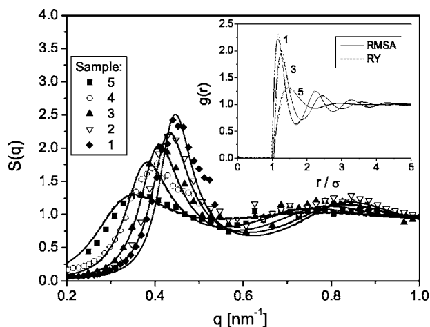
FIG. 6. RY/RMSA fit (solid lines) of the SAXS-determined static structure factors S(q) (symbols) of apoferritin dispersions at five different protein concentrations (samples 1–5). The inset shows the RY/RMSA radial distribution functions of samples 1–3–5. The system parameters of samples 1–5, and the RY and RMSA fitting charges are listed in Table I.
