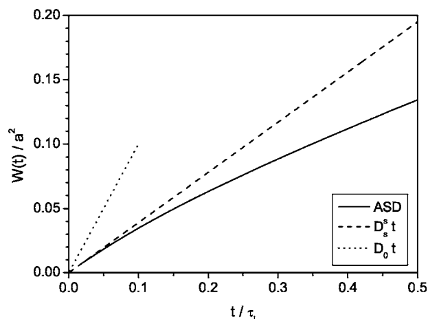
FIG. 5. ASD simulation results, using N=216 particles, for the mean-squared displacement W(t)/a^2 vs reduced time t/\tau_l for \phi=0.327 and Z=28 . Additionally displayed is the short-time asymptotic form D_s(Z, \phi)t (dashed line) in comparison with the mean-squared displacement of noninteracting spheres (dotted line).
