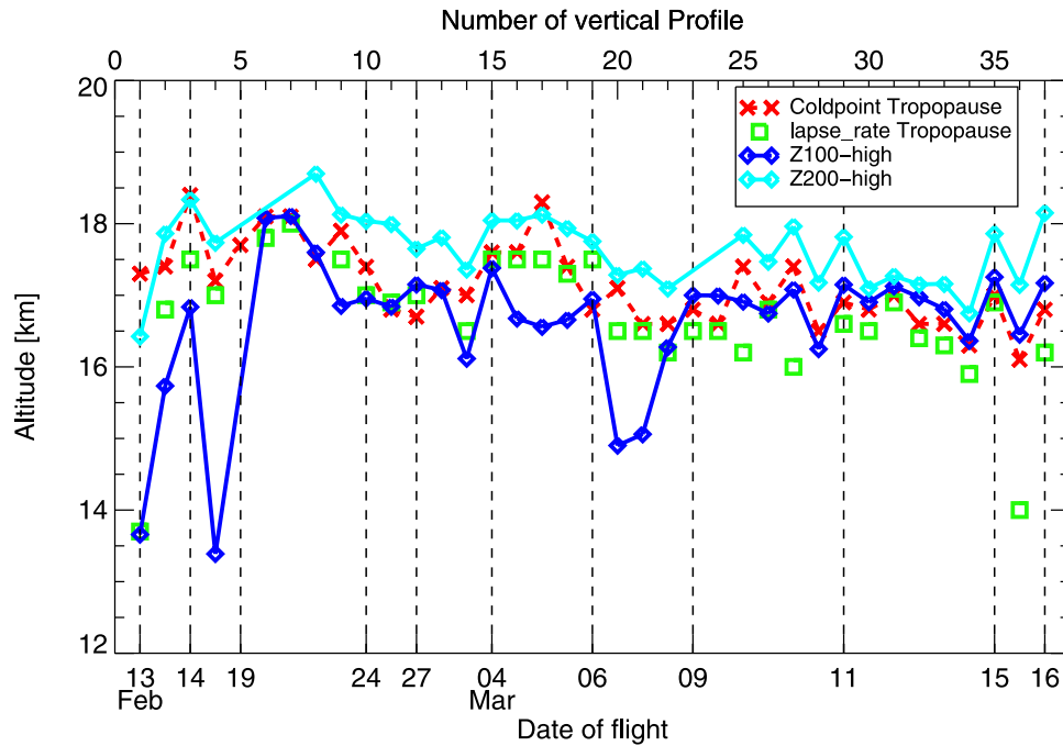
Figure 1. Cold-point tropopause (crosses), lapse-rate tropopause (squares), and the highest pressure-altitudes where 100 and 200 ppbv ozone thresholds were found (diamonds) for all tropical ascents and descents of the APE-THESEO campaign. Profile numbers are as in Table 1.
