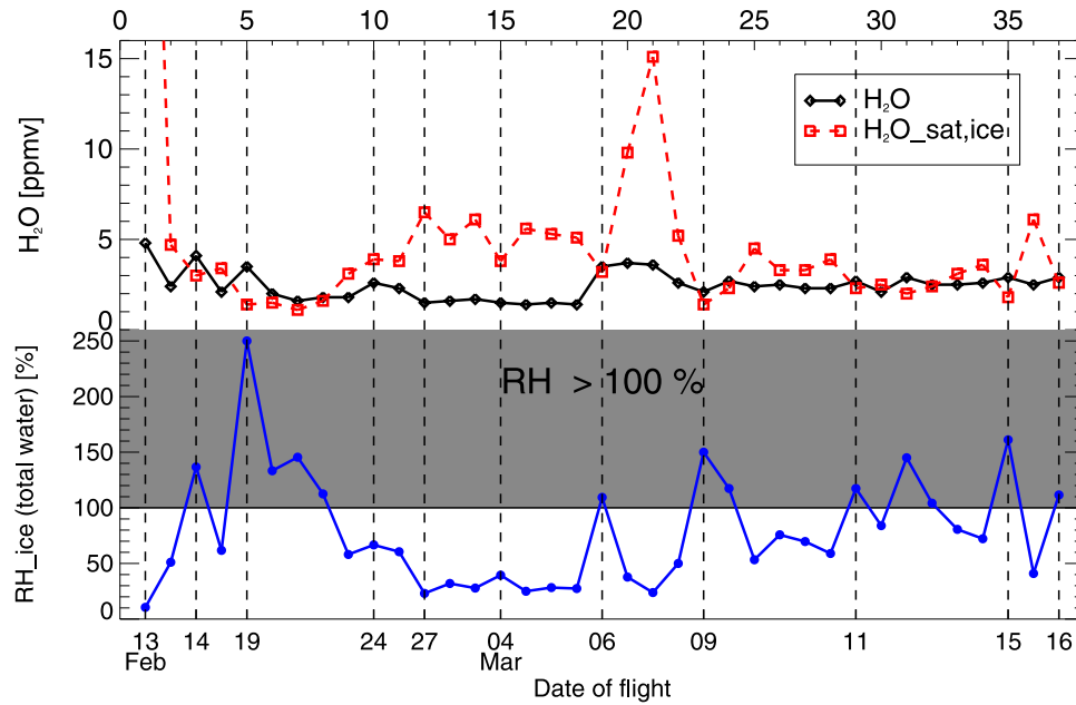
Figure 3. (top) Total water mixing ratio (diamonds) and saturated vapor mixing ratio over ice (squares) at the hygropause for each ascent and descent of the Geophysica across the hygropause. The profiles are the same as those listed in Table 1. (bottom) Relative humidity (RH) over water ice at the hygropause for each ascent and descent of the Geophysica across the hygropause. The region above 100% RH is shaded.
