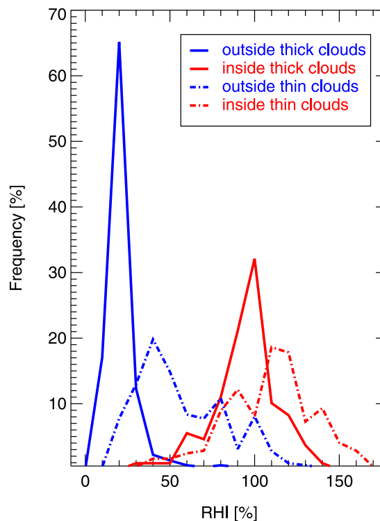
Figure 7. Frequency distribution of relative humidity as measured by FLASH on the flight on 11 March 1999 (solid lines) and on 19 February 1999 (dashed lines), separated for observations inside (red) and outside (blue) clouds.
