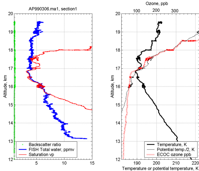
Figure 9. Vertical profiles from an ascent near 11°S on 6 March 1999. (left) MAS backscatter ratio at 532 nm, FISH total water (ppmv), and saturation vapor mixing ratio (ppmv). (right) Temperature (K), potential temperature (K), and ECOC ozone mixing ratio (ppbv). The potential temperature data have been divided by two for ease of plotting.
