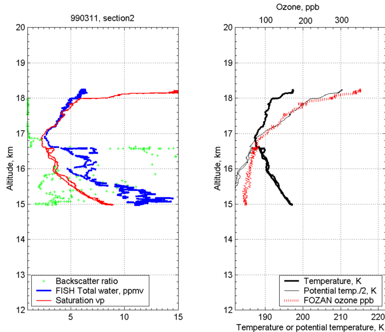
Figure 5. Vertical profiles from an ascent near 14°S on 11 March 1999. (left) Multiwavelength Aerosol Laser Scatterometer (MAS) backscatter ratio at 532 nm, FISH total water (ppmv), and saturation vapor mixing ratio (ppmv). Note that MAS data extend off-scale. The maximum backscatter recorded by MAS on the flight leg was 48, at an altitude of 16.6 km. (right) Temperature (K), potential temperature (K), and FOZAN ozone mixing ratio (ppbv). The potential temperature data have been divided by two for ease of plotting.
