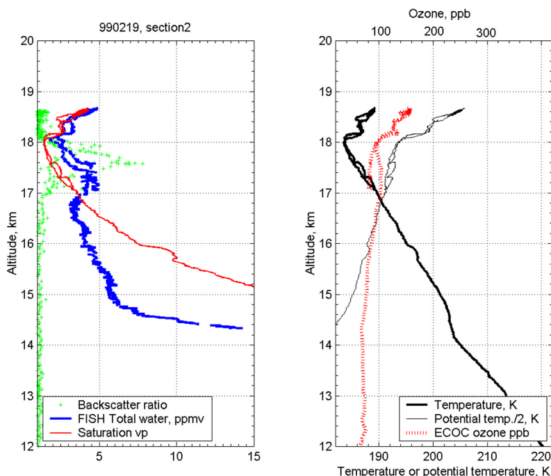
Figure 8. Vertical profiles from a descent near the equator on 19 February 1999. (left) MAS backscatter ratio at 532 nm, FISH total water (ppmv), and saturation vapor mixing ratio (ppmv). (right) Temperature (K), potential temperature (K), and Electro-Chemical Ozone Cell (ECOC) ozone mixing ratio (ppbv). The potential temperature data have been divided by two for ease of plotting.
