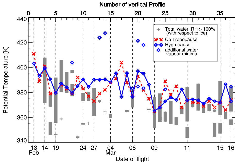
Figure 2. Potential temperature of the cold-point tropopause (crosses) and the hygropause (i.e., the minimum measured total water by FISH) (diamonds) for each ascent and descent of the Geophysica across the hygropause. Additional minima in total water are shown as diamonds. Also shown is the section of each profile that is saturated with respect to water ice (shaded bars).
