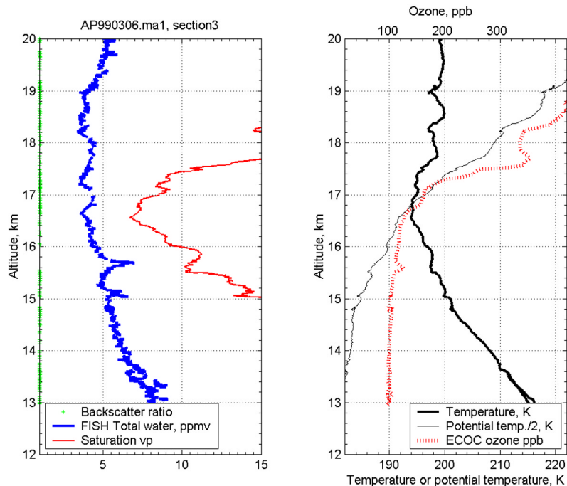
Figure 10. Vertical profiles from an ascent near 18°S on 6 March 1999. (left) MAS backscatter ratio at 532 nm, FISH total water (ppmv), and saturation vapor mixing ratio (ppmv). (right) Temperature (K), potential temperature (K), and ECOC ozone mixing ratio (ppbv). The potential temperature data have been divided by two for ease of plotting.
