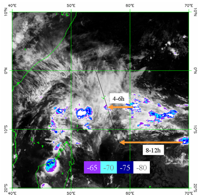
Figure 6. Meteosat 5 infrared cloud image, 5 hours (0116 LT, 2116 GMT) prior to the takeoff of the Geophysica aircraft from the Seychelles (green islands in the center of the plot) on 11 March 1999. The flight path is given as the black line. The aircraft first flew south-southeastward, then returned along the track north-northwestward, overflew Mahé, reached the equator, and then returned south-southeastward. Colors indicate cloud-top height in degrees Celsius (see legend bar). Orange arrows show the transport of recently convected air at 100 hPa in the time intervals shown.
