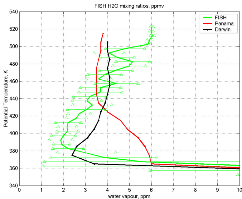
Figure 11. A comparison of the range of water vapor profile from FISH (February–March 1999) with profiles from Darwin [Kelly et al. , 1993], which took place in January and February 1987, and Panama [Kley et al. , 1982], which took place in September 1980. The range bars on the FISH data show \pm 1 standard deviation.
