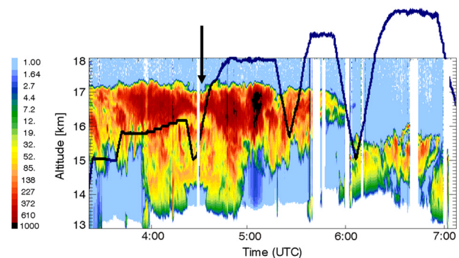
Figure 4. Backscatter ratio (ratio of air plus aerosol to air molecular backscatter intensity) at 1064 nm of the cirrus cloud on 11 March 1999, measured by the lidar on board the Falcon aircraft approximately 1 hour prior to the Geophysica observations; the Geophysica flight track is given by the blue line. The Falcon turned back at 0430 at 14°S; hence the symmetry in the cirrus about the turn point. The aspect ratio is 1:250, i.e., the cloud structures are compressed horizontally by a factor of 250. The vertical profile shown in Figure 5 is marked by the arrow.
