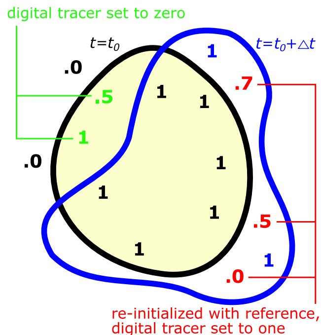
Figure 7. Schematic diagram of the strategy to eliminate cross-vortex mixing from a CLaMS simulation at every time step. On the basis of prior distribution of the vortex tracer Tr_V (black, t = t_0 ) all APs that were advected or mixed into a later vortex (blue solid contour, at t = t_0 + \Delta t ) and therefore have Tr_V < 1.0 (red) are reinitialized with the vortex correlation. Tr_V is reinitialized to zero outside (green) and to one inside the vortex before the next time step.
