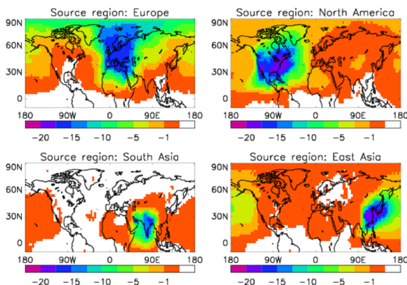
Figure 3. Percentage change in deposition of \text{NO}_y in each \text{NO}_x emission perturbation experiment relative to the control run, using multi-model annual mean deposition fluxes. The annual total deposition fluxes from each model were interpolated onto a 2.5^\circ \times 2.5^\circ grid, from which the multi-model mean values were calculated; the data above are differences in the multi-model means. The white areas indicate a change in deposition of less than 0.1%.
