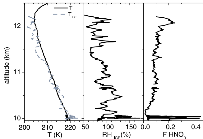
Figure 2. Vertical profile of T , T_{ICE} , RH_{ICE} , and the fraction F of \text{HNO}_{3,\text{tot}} in ice particles ( \text{HNO}_{3,\text{part}}/\text{HNO}_{3,\text{tot}} ). Note that we use a \text{HNO}_3/\text{NO}_y ratio ( R ) of 0.5 for the gas phase ( R = 1 for particles, see text). The cirrus cloud was observed at 58 < RH_{ICE} < 173\% . On average 9% of \text{HNO}_{3,\text{tot}} is contained in ice, increasing to 19% at T < 205 \text{ K} .
