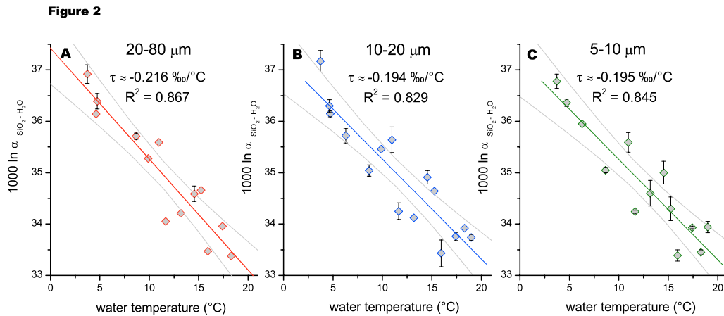
Figure 2. Dependency of the oxygen isotope fractionation in biogenic opal on temperature for three different size classes of freshwater diatoms from Lake Holzmaar. Each symbol represents the average of up to 4 measurements. Error bars represent 1\sigma . Centre lines are regression lines; neighbouring curves express 95% confidence intervals. Regression coefficients are identical at p < 0.05 .
