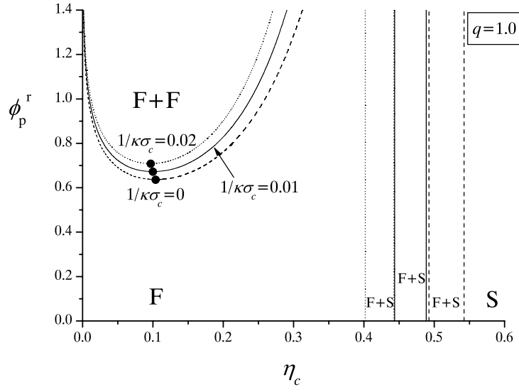
Figure 7. Same as figure 5 but for q = 1.0 . F + F denotes the stable fluid-fluid coexistence region.
