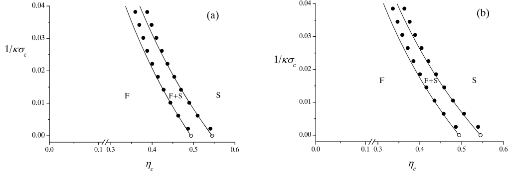
Figure 3. Fluid-solid (fcc) transition of charged colloidal spheres interacting with a hard-core repulsive Yukawa potential (1) with a) \beta\epsilon = 20 and b) \beta\epsilon = 39 . Open symbols denote simulation results of pure hard spheres taken from Ref. [60]. Filled circles denote the simulation results of Hynninen and Dijkstra [59]. Full curves correspond to the theoretical predictions as described in section 3.
