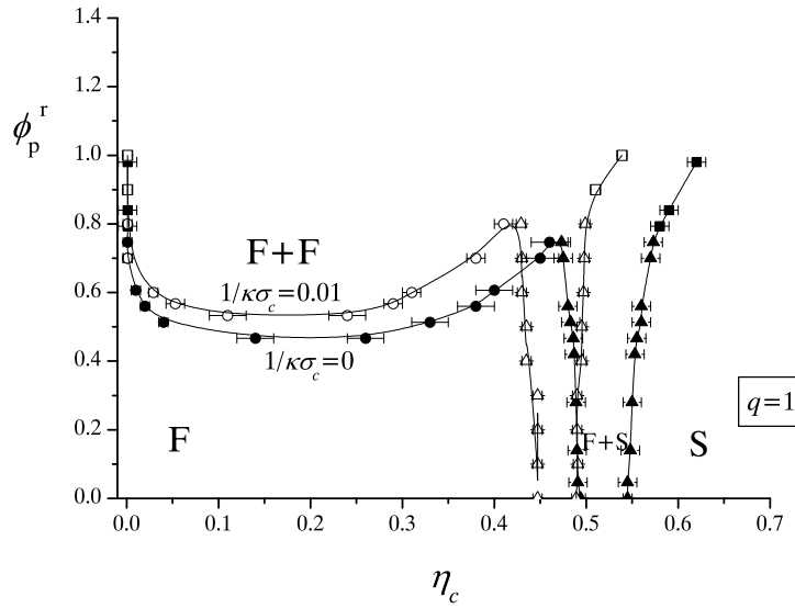
Figure 13. Same as figure 11, but for q = 1 . F + F denotes the stable fluid-fluid coexistence region.
