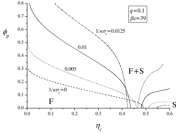
Figure 9. Same as figure 8, but with \beta\epsilon = 39 .
