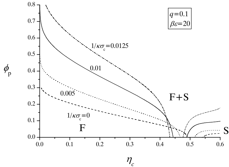
Figure 8. Same as figure 5 but as a function of the actual ideal polymer concentration \phi_p .
