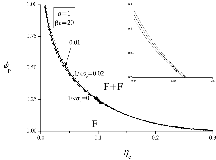
Figure 10. Same as in figure 8, but with size ratio q = 1.0 . The filled circles indicate the location of the gas-liquid critical points. The inset is a blow-up of the critical region of the liquid-gas binodal.
