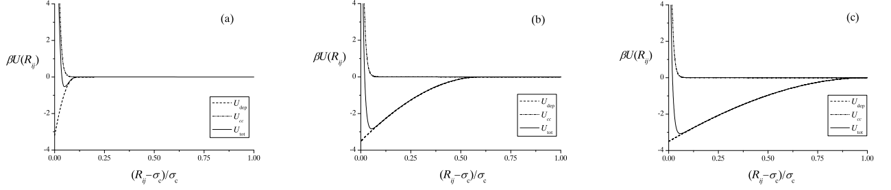
Figure 1. Pair interaction between two colloidal spheres with hard-core diameter \sigma_c interacting with a Yukawa pair potential U_{cc} (equation 1) and an effective depletion interaction U_{dep} (equation 5) due to the presence of non-adsorbing polymer coils with an effective diameter \sigma_p . The total effective interaction U_{tot} (equation 6) is denoted by the full curve. The Yukawa repulsion is characterised by \beta\epsilon = 20 and \kappa\sigma_c = 100 . The depletion interaction are: a) for a size ratio q = \sigma_p/\sigma_c = 0.1 and relative polymer concentration \phi_p^r = 0.2 , b) q = 0.6 and \phi_p^r = 1 , and c) q = 1 and \phi_p^r = 1.4 .
