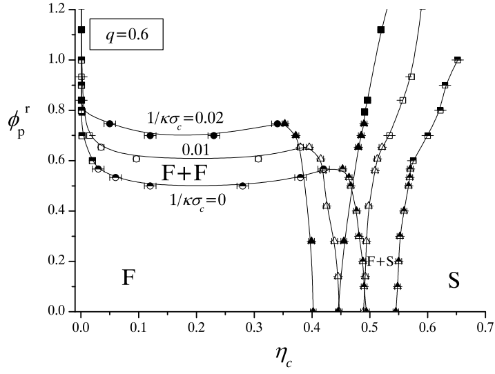
Figure 12. Same as figure 11, but for q = 0.6 . F + F denotes the stable fluid-fluid coexistence region.
