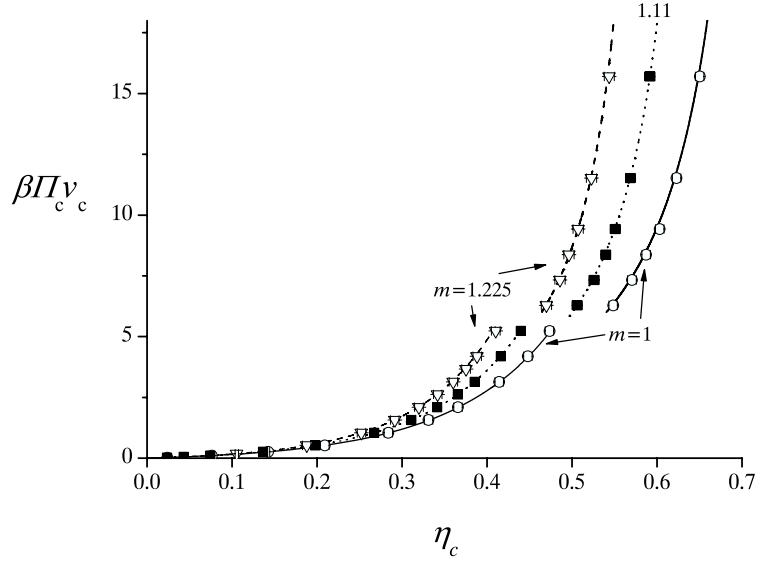
Figure 2. Pressure of a dispersion of charged colloidal spheres interacting with U_{cc}(R_{ij}) (see equation (1)) for \beta\epsilon = 20 and 1/\kappa\sigma_c = 0 (open circles, full curves), 0.01 (filled squares, dotted curves), and 0.02 (open triangles, dashed curves), corresponding to m = 1, 1.110 , and 1.225 , respectively, in equation (7). The symbols denote the simulation results, while the curves denote the theoretical predictions of equations (11) (lower set of pressures) and (12) (upper set).
