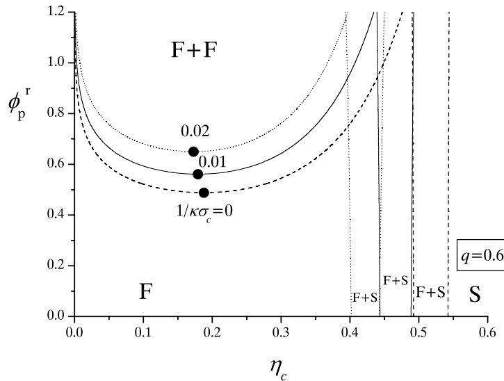
Figure 6. Same as figure 5 but for q = 0.6 . F + F denotes the stable fluid-fluid coexistence region.
