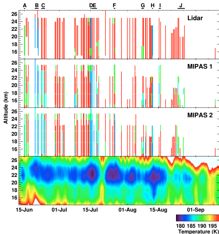
Fig. 10. Comparison between lidar and MIPAS PSC type analysis. For lidar, red indicates Type 1a, green Type 1b and blue Type 2 PSC. In case of MIPAS red stands for R1, blue for R3, green for R2, and blue-green for region R4 in Fig. 9. “MIPAS 1” indicate the nearest and “MIPAS 2” the second nearest MIPAS limb-scan with respect to the lidar observation in terms of \Delta t_{\text{tot}} (see text). A–J denote periods discussed in the text.
