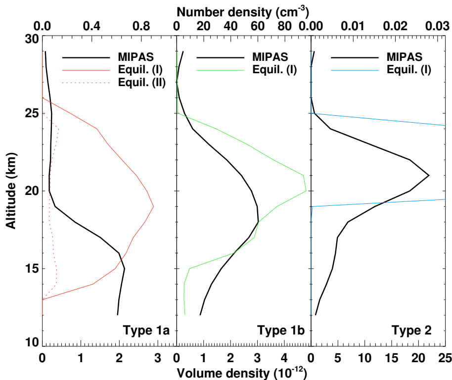
Fig. 7. MIPAS PSC retrieval of number density (black curves, top axis) for the collocations with the three different Lidar Type measurements. The results were obtained with the following settings of median radius and refractive indices. Type 1a: r_m = 0.8 \mu\text{m} , \beta -NAT refractive indices by Biermann (1998) and this work; Type 1b: r = 0.2 \mu\text{m} , refractive indices by Biermann et al. (2000) ; Type 2: r = 5.0 \mu\text{m} , refractive indices by Toon et al. (1994) . Volume density is calculated from N, r_m , and \sigma = 1.35 (black curves, bottom axis). Colored curves are volume density profiles for NAT (red), STS (green), and ice (blue) in thermodynamic equilibrium (see text for details).
