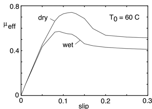
FIG. 11. The effective friction coefficient as a function of slip for dry and wet road surfaces, calculated for a standard tread compound and an asphalt substrate.
