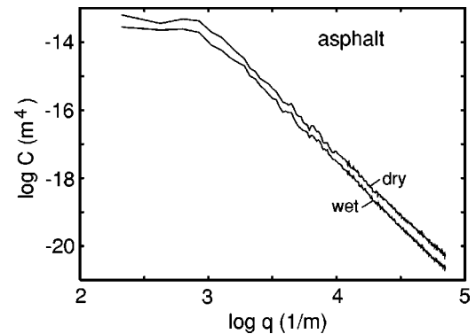
FIG. 9. The logarithm of the surface roughness power spectra C(q) for a dry and a wet asphalt road surface, as a function of the logarithm of the wave vector q .
