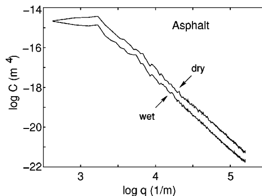
FIG. 3. The logarithm (to base 10) of the surface roughness power spectra C(q) for a dry and a wet asphalt road surface, as a function of the logarithm of the wave vector q .
