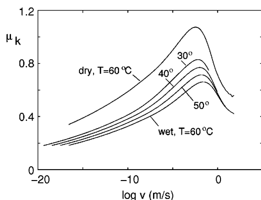
FIG. 5. Kinetic friction coefficient as a function of the logarithm of the sliding velocity, calculated for a standard tread compound and an asphalt substrate.
