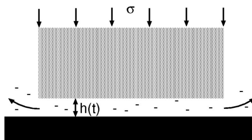
FIG. 6. A tread block squeezed against a smooth flat substrate in a liquid. The surface separation h(t) decreases with increasing time.
