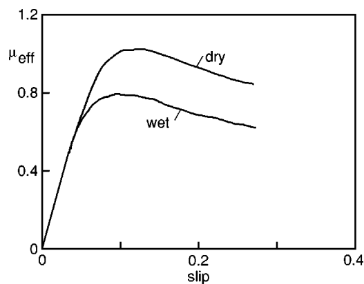
FIG. 1. A typical measured effective friction coefficient as a function of slip for dry and wet road surface. See Sec. III for the definition of the slip.
