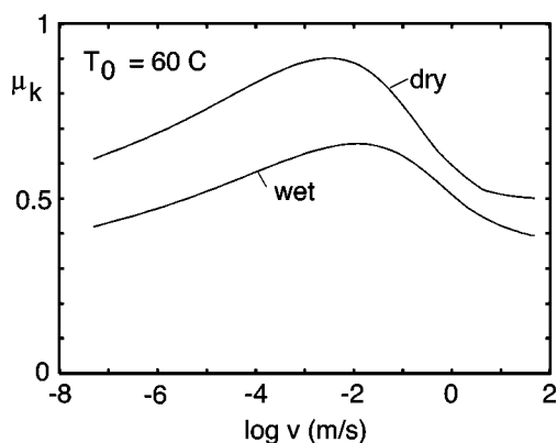
FIG. 10. Kinetic friction coefficient as a function of the logarithm of the sliding velocity, calculated for a standard tread compound and an asphalt substrate.
