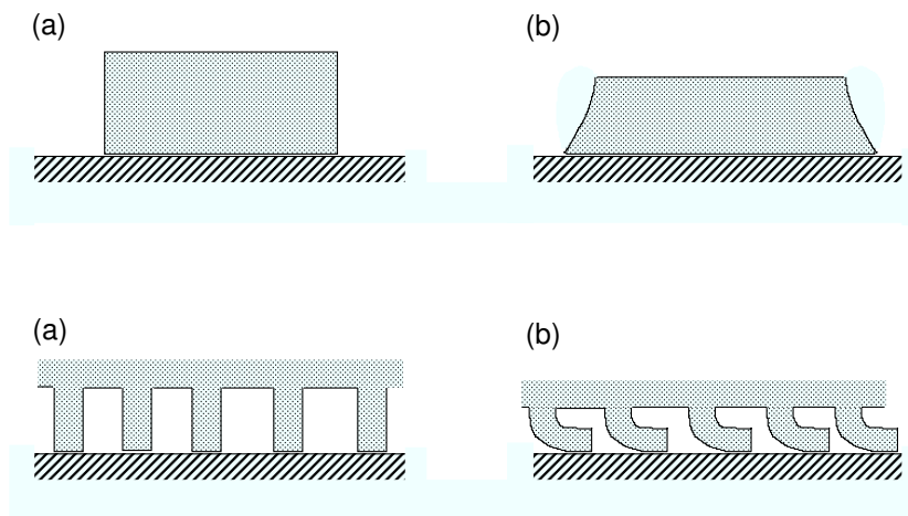
Figure 47. Elastic deformation of a rubber block with a smooth surface (top) and a structured surface (bottom). (a) shows the initial state before applying a squeezing force, and (b) the new state (without load) after applying (and then removing) a very large squeezing force. In state (b) a large elastic energy is stored in the rubber which is “given back” during pull-off resulting in a nearly vanishing pull-off force.
