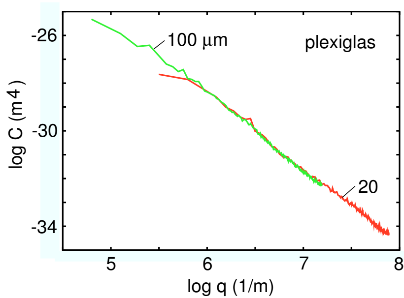
Figure 17. The surface roughness power spectra C(q) for a plexiglas surface. The two curves are based on the height profiles measured with an AFM at two different spatial resolution over 20 \times 20 and 100 \times 100 \mu\text{m} square areas.
