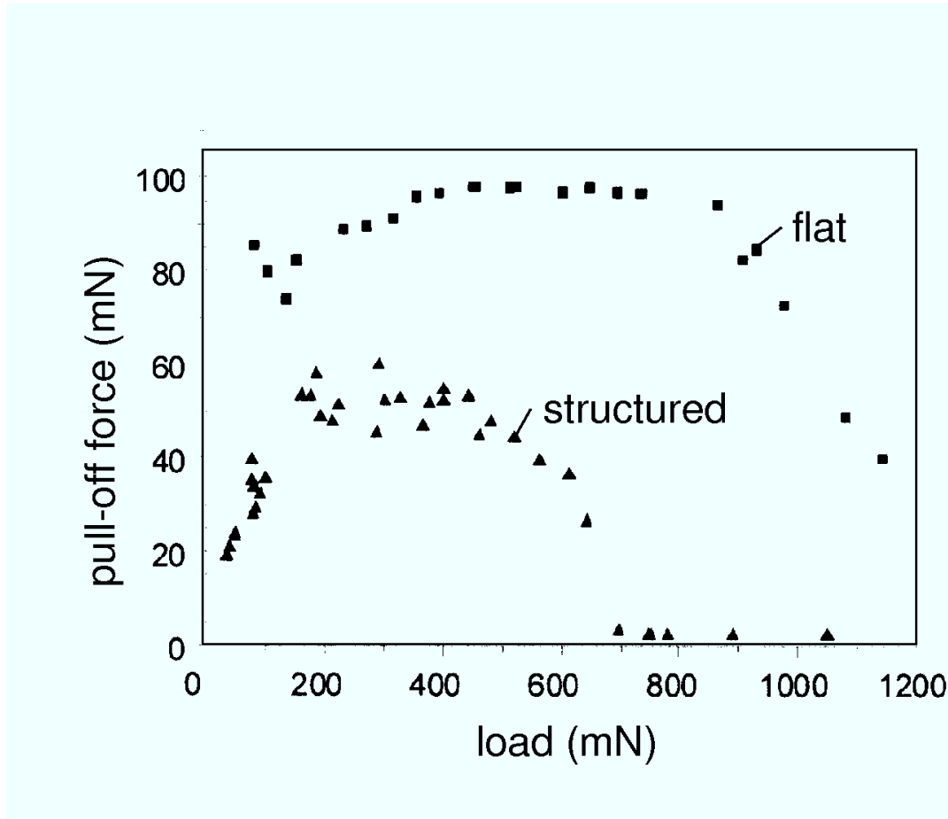
Figure 46. The pull-off force as a function of the squeeze force or load, for silicon rubber in contact with a smooth glass surface. From Ref. [71].
