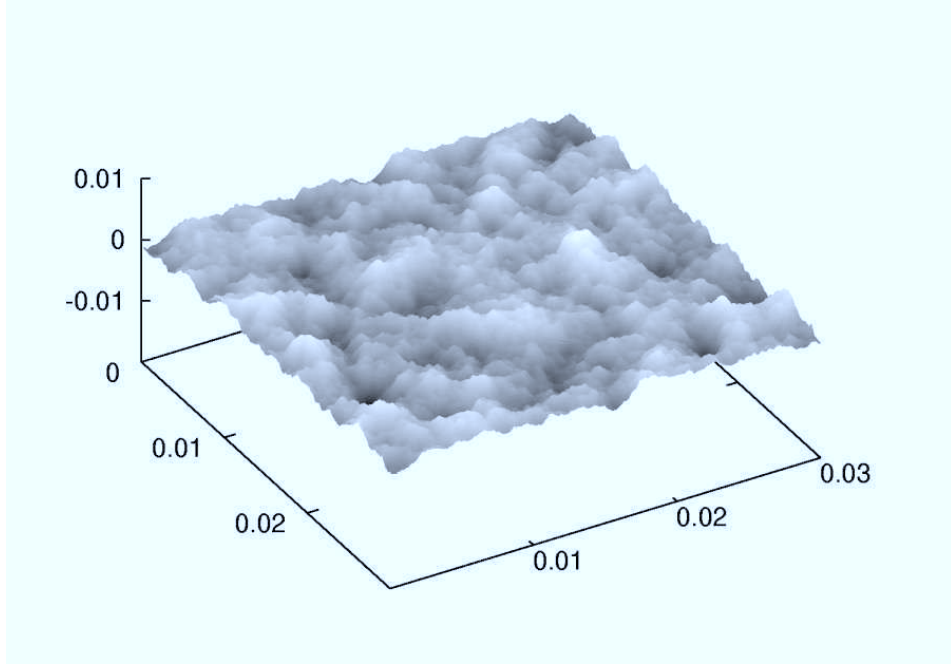
Figure A1. Computer generated rough substrate. The surface has root mean square roughness 0.001 m, roll-off wave vector q_0 = 1000 \text{ m}^{-1} , and Hurst exponent H = 0.8 . Length in the picture are in meters.
