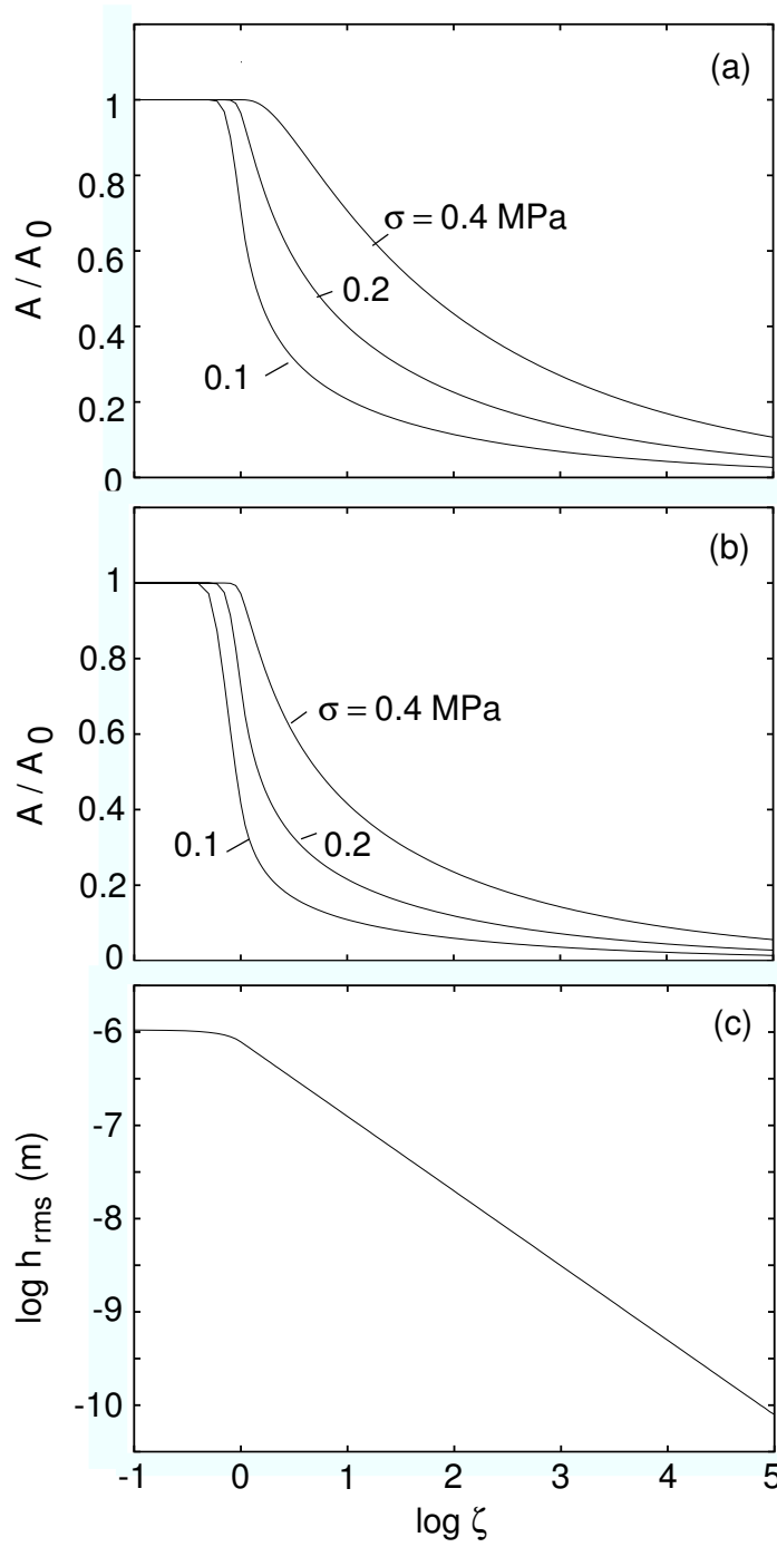
Figure 30. Calculated relative contact area after one second of contact for tread tire rubber (a), for rim tire rubber (b), and the root-mean-square roughness as a function of magnification (c), where \zeta = 1 corresponds to a wavelength \lambda_0 = 2\pi/q_0 \approx 100 \mu\text{m} . The highest magnification \zeta = 10^5 corresponds to \lambda \approx 1 \text{ nm} . Results are shown for a nominal pressures \sigma_0 = 0.1, 0.2 and 0.4 \text{ MPa} , at the temperature T = 60^\circ\text{C} . Substrate surface with rms roughness h_0 = 1 \mu\text{m} and roll-off wave vector q_0 = 6 \times 10^4 \text{ m}^{-1} .
