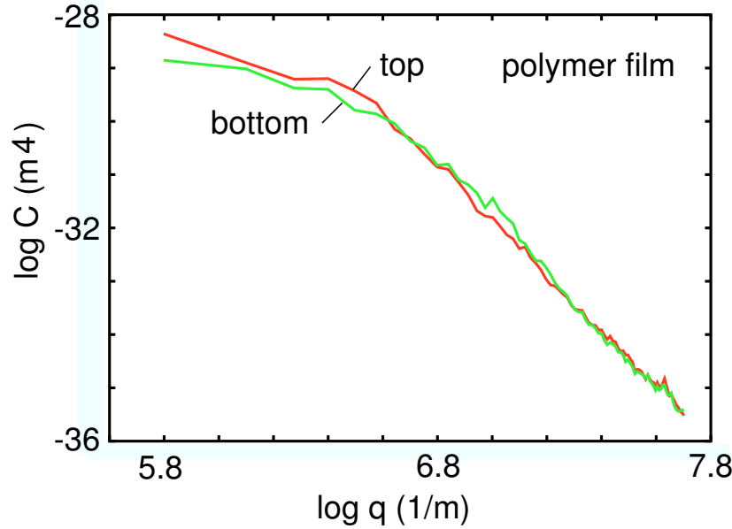
Figure 19. The top C_T^* and the bottom C_B^* surface roughness power spectra for a polymer film spin coated on a very smooth substrate and dried. From Ref. [13].
