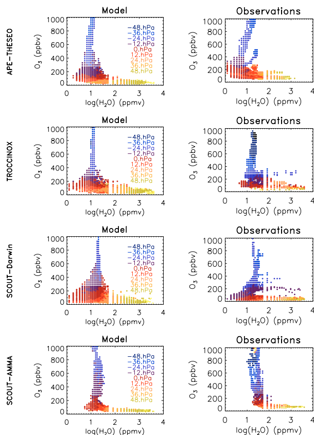
Fig. 8. \text{H}_2\text{O} - \text{O}_3 correlations for ECHAM5/MESSy (left column) and the observations (right column), relative to the regions and time periods of APE-THESIO, TROCCINOX, SCOUT-Darwin, and SCOUT-AMMA campaigns (from top to bottom), divided by color according to 12 hPa-thick pressure ranges whose central value is indicated in the legend.
