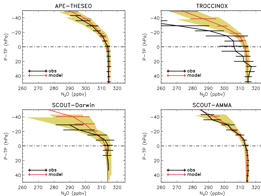
Fig. 6. The same as Fig. 3, for N 2 O.
