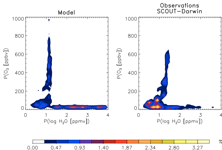
Fig. 9. Joint probability distribution functions (PDFs) of the \text{H}_2\text{O} - \text{O}_3 correlation for the region and time period relative to the SCOUT-Darwin campaign. Left: ECHAM5/MESSy; right: observations.
