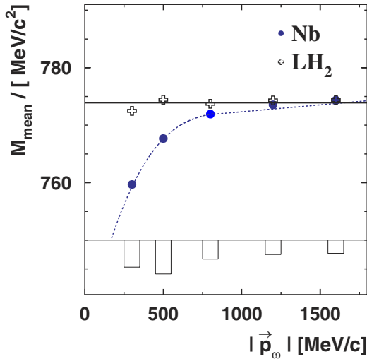
FIG. 4 (color online). Mean value of the \pi^0\gamma invariant mass as a function of the \omega momentum at an estimated average density of 0.6\rho_0 for the Nb data (circles) and the \text{LH}_2 (crosses) along with a fit. The systematic errors are determined by varying the integration range of 0.65 \text{ GeV}/c^2 < M_{\pi^0\gamma} < 0.9 \text{ GeV}/c^2 by 50 \text{ MeV}/c^2 and are shown as a bar chart for the Nb data. In contrast to the peak positions, the mean values do not reach the nominal vacuum mass of 782 \text{ MeV}/c^2 due to the detector response function.
