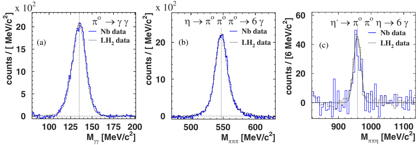
FIG. 1 (color online). Background subtracted invariant mass distributions for the long-lived mesons \pi^0 , \eta , and \eta' . The solid and dashed histograms correspond to data taken with a Nb and \text{LH}_2 target, respectively. The meson line shapes are reproduced by Monte Carlo simulations, as demonstrated for the \eta' signal (solid curve).
