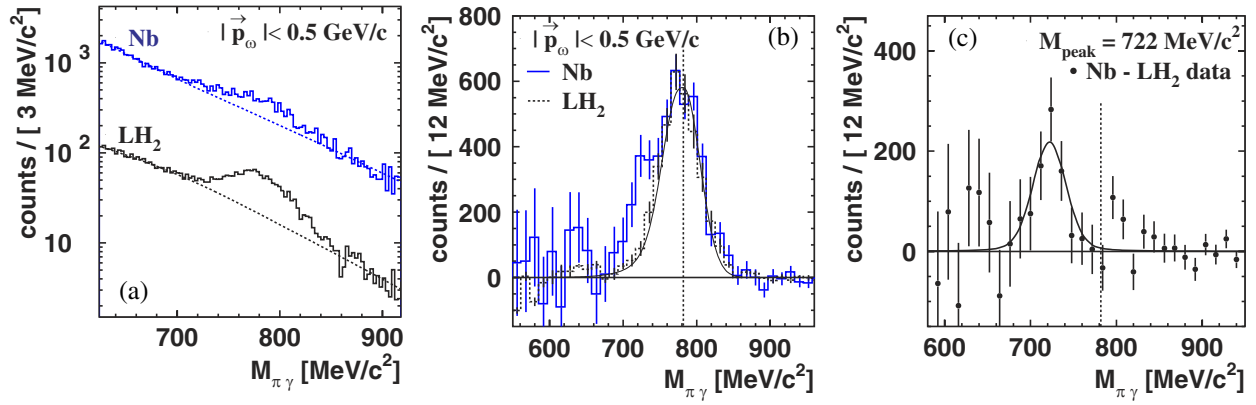
FIG. 2 (color online). (a) Inclusive \pi^0\gamma invariant mass spectra for momenta less than 500 MeV/c. Upper histogram: Nb data, lower histogram: \text{LH}_2 target reference measurement. The dashed lines indicate fits to the respective background. (b) \pi^0\gamma invariant mass for the Nb data (solid histogram) and \text{LH}_2 data (dashed histogram) after background subtraction. The error bars show statistical uncertainties only. The solid curve represents the simulated line shape for the \text{LH}_2 target. (c) In-medium decays of \omega mesons along with a Voigt fit to the data (see text). The vertical line indicates the vacuum \omega mass of 782 MeV/c 2 .
