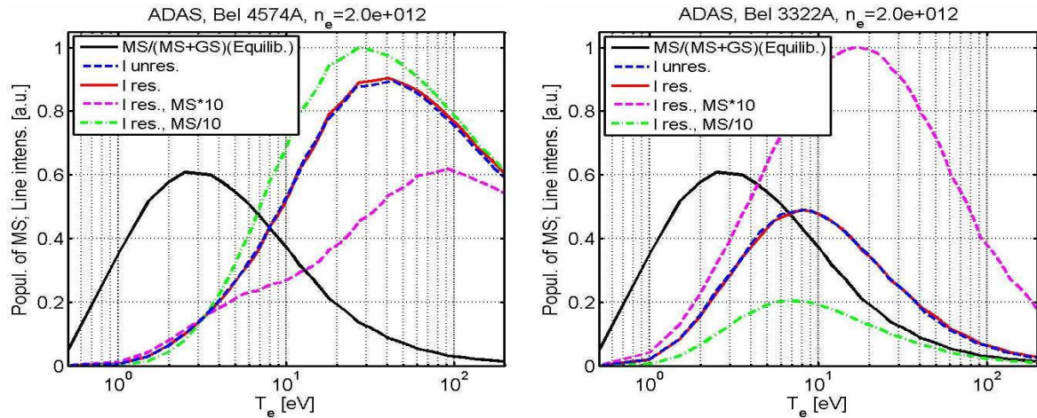
Fig.3. ‘Equilibrium approach’ illustration: relative MS population and respective line intensities in MS resolved (“I res.”) and unresolved (“I unres.”) cases; singlet (left) and triplet (right) lines.
