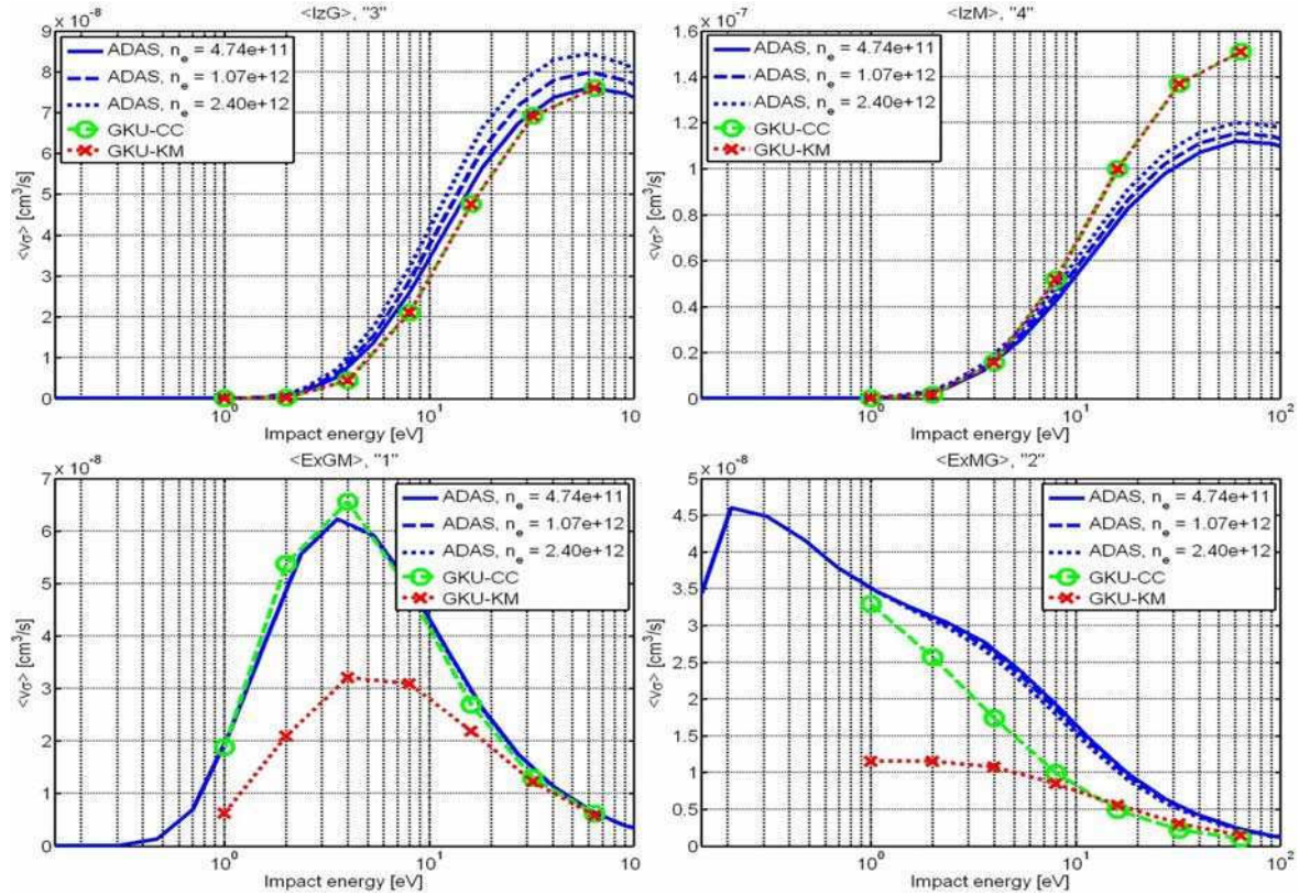
Fig.2. Comparison of effective rates produced by ADAS and GKU. “ \langle I_z G \rangle ”, “ \langle I_z M \rangle ” – ionization from GS and MS; “ \langle ExGM \rangle ” – transition GS \rightarrow MS ; “ \langle ExMG \rangle ” – transition MS \rightarrow GS . GKU code uses 2 sets of underlying data – calculated in K-matrix (“GKU-KM”) and CCC (“GKU-CC”) approaches.
