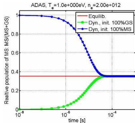
Fig.4. Time evolution of MS population-“dynamic approach” (“Dyn.”) with different initial conditions converging to the equilibrium approach obtained value (“Equilib.”)
