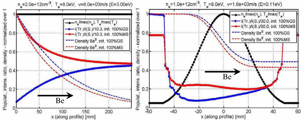
Fig.5. Profiles along narrow monoenergetic Be beam. Constant (left) and Gaussian (right) background plasma profile. Ratio of triplet 3322A to singlet 4573A line (“ I(tr.)/I(S.) ”) and neutral Be density for 2 extreme assumptions of initial population (“100%GS”, “100%MS”).
