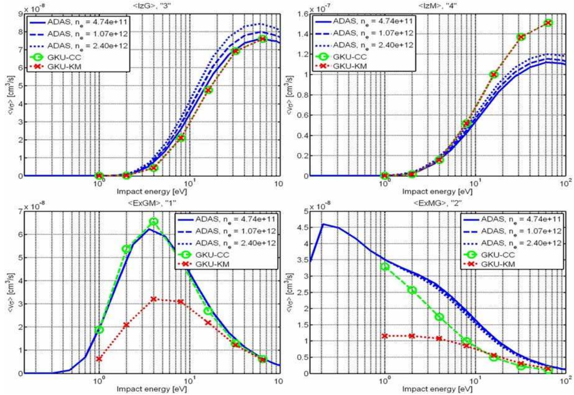
Fig.2. Comparison of effective rates produced by ADAS and GKU. “ \langle I_{zG} \rangle ”, “ \langle I_{zM} \rangle ” – ionization from GS and MS; “ \langle ExGM \rangle ” – transition GS \rightarrow MS ; “ \langle ExMG \rangle ” – transition MS \rightarrow GS . GKU code uses 2 sets of underlying data – calculated in K-matrix (“GKU-KM”) and CCC (“GKU-CC”) approaches.
