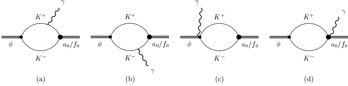
Fig. 1. Diagrams contributing to the radiative decay amplitude (1).
