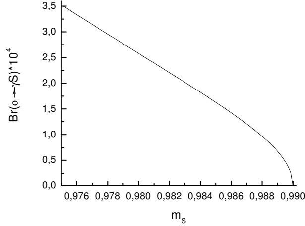
Fig. 3. The dependence of the branching Br(\phi \rightarrow \gamma S) on the mass of the scalar meson in the molecular model.
