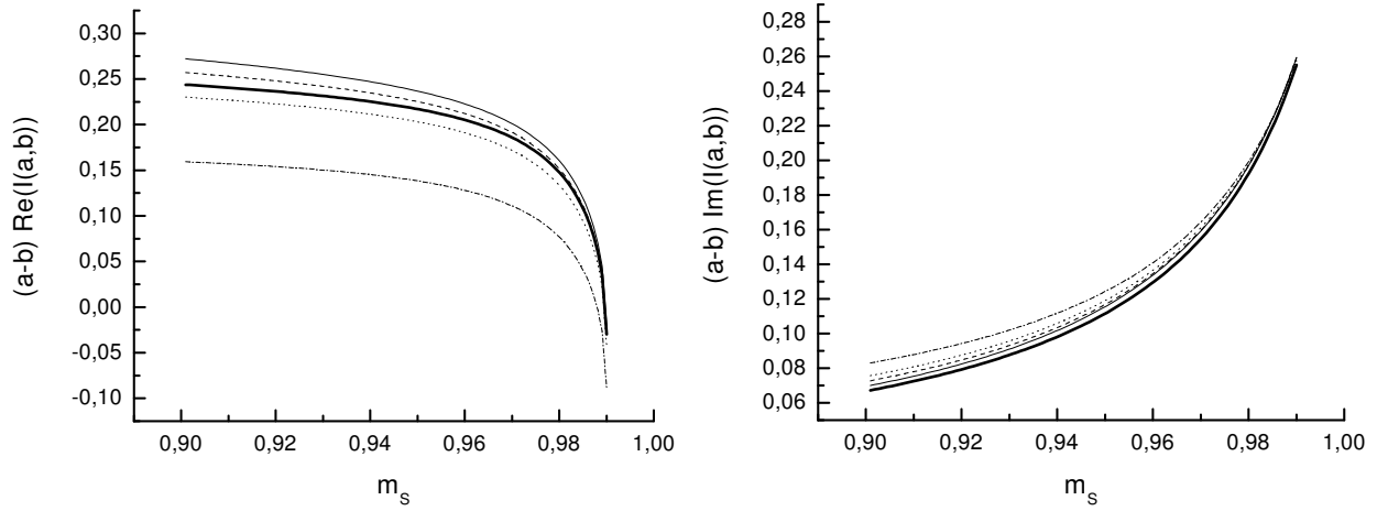
Fig. 2. The real (the left plot) and the imaginary (the right plot) parts of the function I_1 = (a - b)I(a, b; \Gamma) for \beta = 0.2 GeV (dash-dotted line), \beta = 0.4 GeV (dotted line), \beta = 0.6 GeV (dashed line), and \beta = 0.8 GeV (thin solid line). The result of the full pointlike theory is given by the thick solid line.
