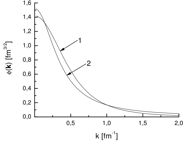
Fig. 4. The wave function of the K\bar{K} system, in momentum space. The approximate solution Eq. (28) — the curve 1, and the deuteronlike wave function, Eq. (23) — the curve 2.
