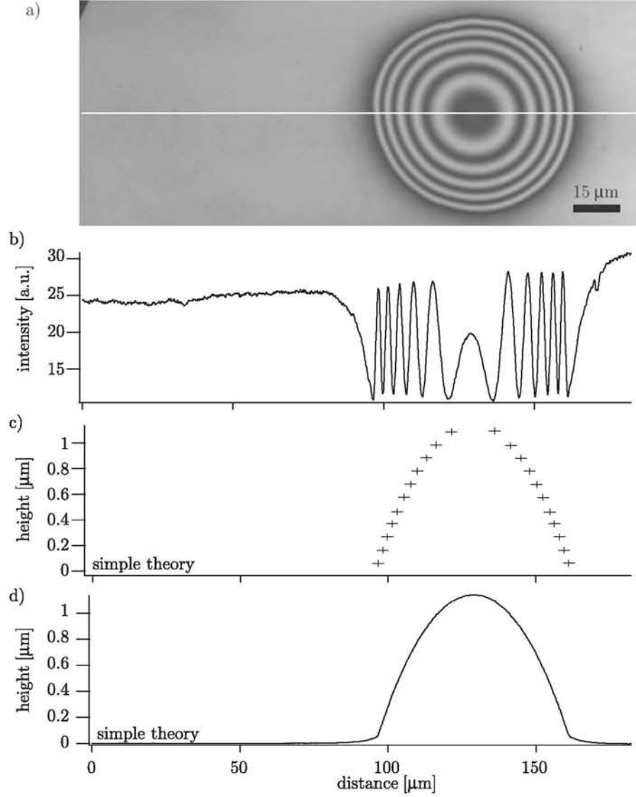
Figure 5.14: a) Raw image of a RICM micrograph of a drop of fluid PDMS on a thin film of cross-linked PDMS under water. b) Intensity profile I(x) along the white line in the RICM micrograph. c) Single heights h can be reconstructed from the extreme values according to the simple theory, Eq. 5.38. Note that the height has an unknown offset of N \cdot \Delta h . d) Using the simple theory, the height profile within the intervals can be analyzed by an inverse cosine function (compare Eq. 5.39).
