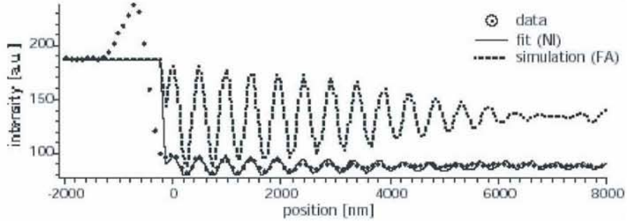
Figure 5.26: Intensity plot from a RICH interferogram of a water droplet on a glass substrate exposed to air. The measured data were fitted by the theory of non-planar interfaces (NI / drawn line) and the finite aperture theory (FA / dashed line), respectively. The rim caustic can be clearly seen as an intensity overshoot between the plateau of the background region and the sinusoidal intensity profile of the drop region. (from [Wiegand et al., 1998]).
