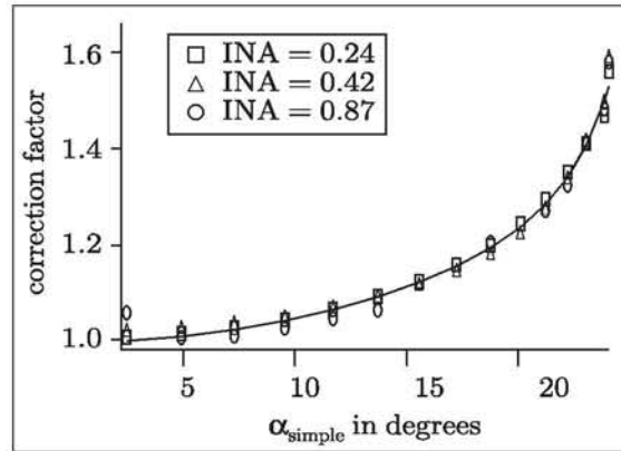
Figure 5.18: Non-local theory correction factors for the height profile reconstruction. The drop shape is modelled as a simple wedge with zero curvature. The correction factor is strongly dependent on the wedge angle but only weakly dependent on the illumination aperture. The continuous line represents a function which was used to determine the correction factor in calculations.
