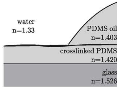
Figure 5.2: Refractive indices of the used system. Measurements of the refractive index of pure PDMS oil and the used PDMS mixtures showed no difference and confirmed the manufacturer's data. The refractive index of the cross-linked polymer was measured by ellipsometry to be 1.4196 \pm 0.0014 (at 632.8 nm). The value for glass cover slides was taken from the glass manufacturer (SCHOTT, Mainz, Germany), the respective value for water from literature [Gerthsen, 1997].
