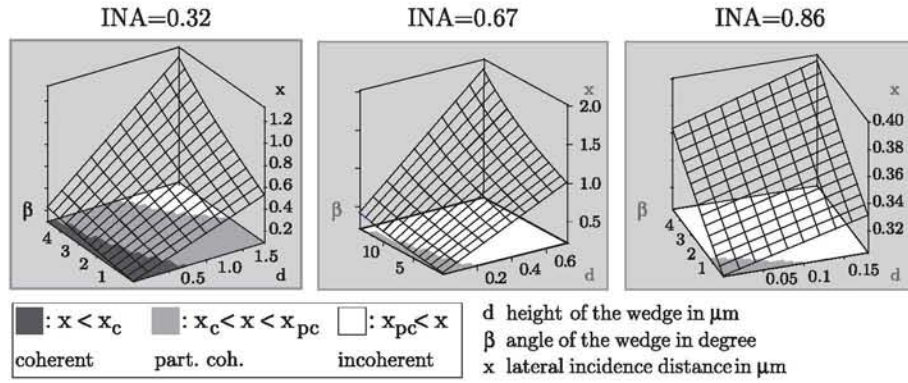
Figure 5.9: Calculation of the maximal possible lateral incidence distance x between two interfering rays for different angles \alpha_{max} = \arcsin(\text{INA}/n) of incident light (see Fig. 5.8(b)). If x is smaller than the lateral coherence length x_c , the visibility S (see Eq. 5.11) of the interference fringes will be maximal. If x is larger than the lateral coherence length x_c the visibility S will decrease.
