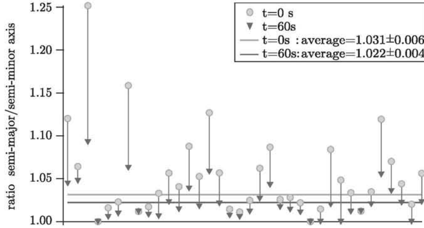
Figure 5.22: The ratio a/b of semi-major axis a to semi-minor axis b is plotted at two different times for all experiments. As can be seen, this ratio deviates only slightly from one, therefore all drops can be regarded as mainly spherical. Moreover, any distortion from the spherical shape will decrease significantly within short times (see plotted values for t = 0\text{ s} and t = 60\text{ s} ).
