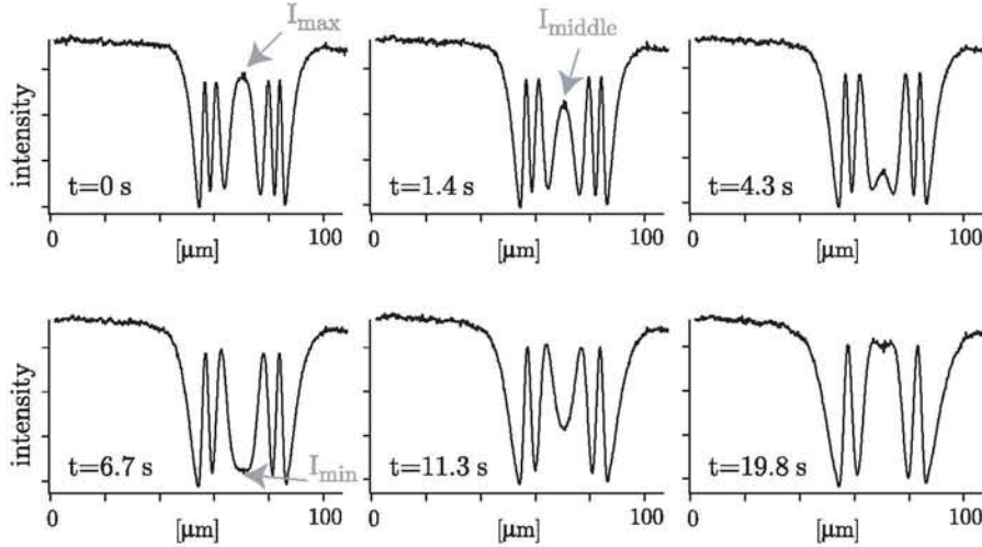
Figure 5.17: Time series of RISM intensity profiles of an evolving drop. The intensity I_{middle} of the middle extremum oscillates between I_{min} or I_{max} .
