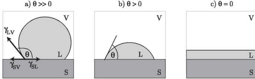
Figure 3.1: Sketch of a small droplet in equilibrium on a solid surface. The contact angle \Theta depends on the interfacial energies \gamma_{ij} via the Young equation (Eq. 3.5). The situation in a) and b) is called partial wetting, c) is referred to as complete wetting with a contact angle of \Theta = 0^\circ .
