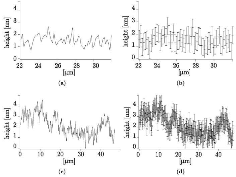
Figure 4.8: RICH height reconstruction profile of a film of cross-linked PDMS on glass immersed in water with ((b) and (d)) and without error bars ((a) and (c)).
