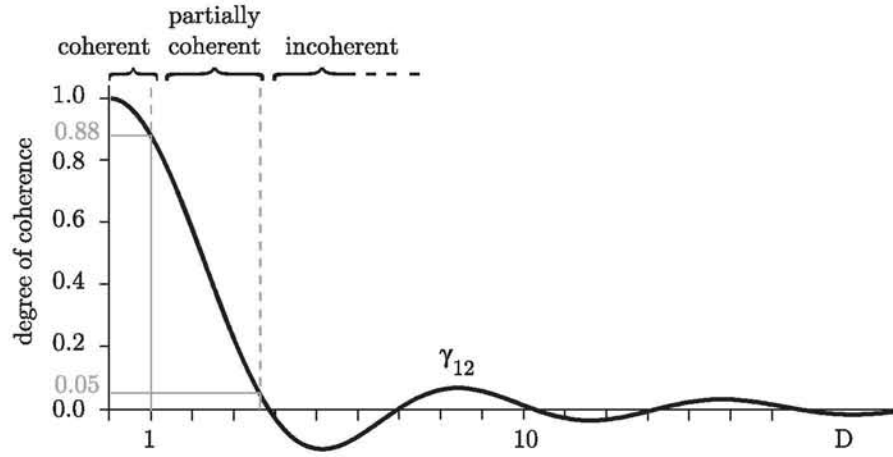
Figure 5.6: Degree of coherence between two points P_1 and P_2 illuminated by a circular light source: \gamma_{12}(D) = \frac{2J_1(D)}{D} .
