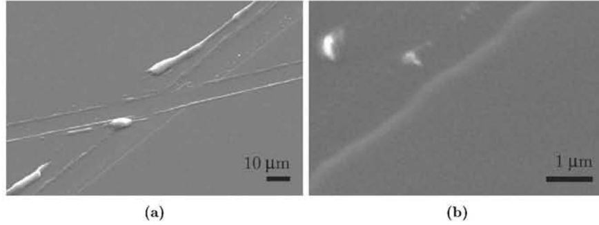
Figure 4.4: SEM micrograph of a film of cross-linked PDMS on glass. The surface appears to be very smooth.
