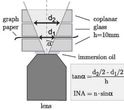
Figure 5.7: Sketch of the method for determining the illumination numerical aperture. Three pieces of coplanar glass of height h = 10\text{ mm} were put on top of the lens. The diameter of the light cone d was determined at the two faces of the middle glass pane. This was done by alternately placing a piece of graph paper in between the respective panes and then measuring the diameter of the clearly visible light cone. The numerical aperture was then calculated according to the shown equations.
