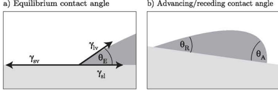
Figure 2.1: a) Static contact angle between solid S , liquid L and vapour V as described by Young's Law: \gamma_{LV} \cos \theta_E = \gamma_{SV} - \gamma_{LS} , where \gamma is the interfacial free energy between the respective substances (s: solid, l: liquid, v: vapour).
