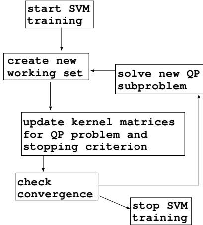
Figure 1: Decomposition scheme for SVM training.
