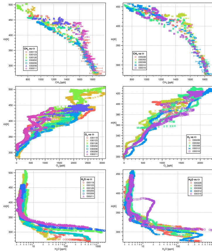
Fig. 2. Mixing ratios of CH 4 (HAGAR), O 3 (FOX) and H 2 O (FISH) plotted versus the potential temperature for all EuPLEX (left panel) and AVC flights (right panel). Error bars denote the precision of the measurement. For O 3 the precision is 10%, for H 2 O 0.3 ppm.
