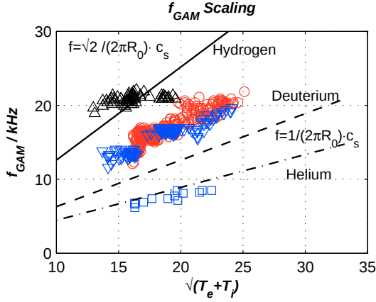
Figure 3: Scaling of the GAMs with \sqrt{T_e + T_i} . The different fits are due to different ion mass. ( \square ) denotes the predominately Helium and ( \triangle ) the Hydrogen plasmas. Other symbols denote Deuterium plasmas with different H/D-ratios.
