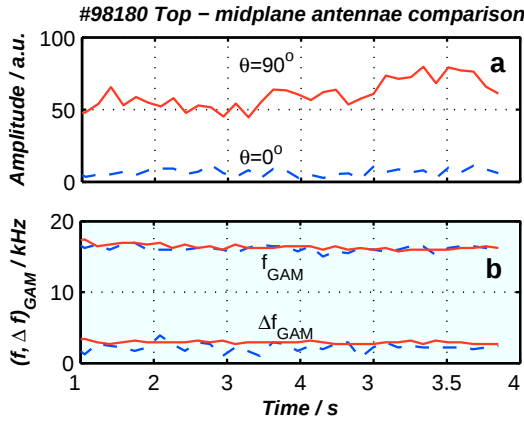
Figure 5: (a) Comparison of the GAM–amplitude at top (solid) and midplane (dashed) position. (b) Center frequency and FWHM of the GAM peak, showing that top and midplane antennae observe the same phenomena.
