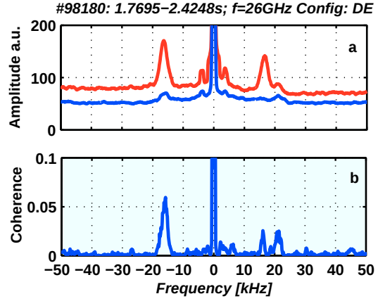
Figure 6: Far poloidal correlation over \Delta\theta = 90^\circ . The GAM is visible in amplitude (a) and coherency (b) spectra at \approx 17 kHz. Beside the GAM a high frequency satellite is observed in the right wing of the spectrum.
