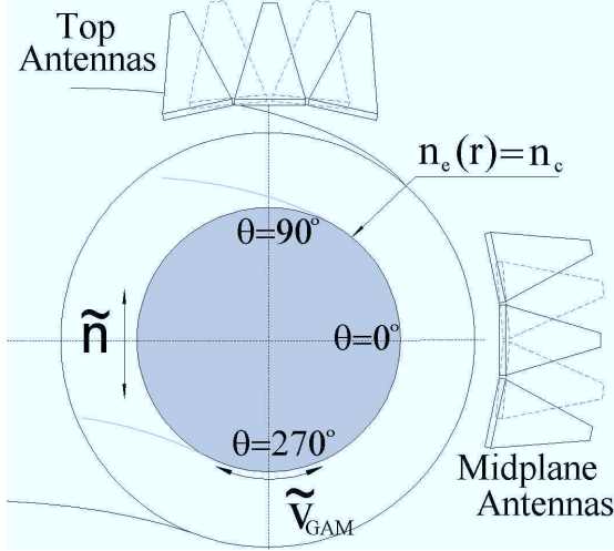
Figure 1: Poloidal cross section with reflectometer antennae and a sketch of the velocity ( \tilde{v}_{GAM} ) and density ( \tilde{n} ) oscillations due to the GAM.
