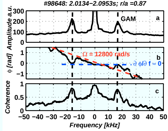
Figure 2: Spectra of amplitude (a), cross phase (b) and coherence (c) obtained from two top antennae. In (a) and (c) a single peak at 16.7 kHz is seen. In (b) the change of the average slope by the GAM is shown.
