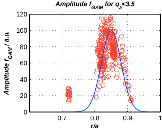
Figure 4: The amplitude of the GAM as obtained from the amplitude spectrum versus r/a . To guide the eye, the localization can be described by Gaussian function (blue curve) centered at r/a = 0.85 .
