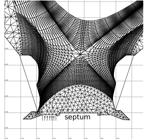
Figure 3: Computational grid and structure for the JET model
