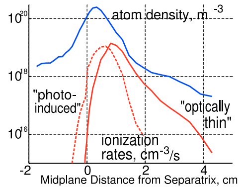
Figure 5: "Optically thin" and "photo-induced" ionization rates in front of the inner target
