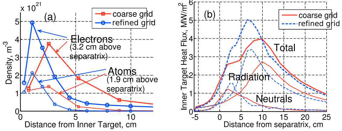
Figure 2: Influence of the grid resolution on the results of the calculations
