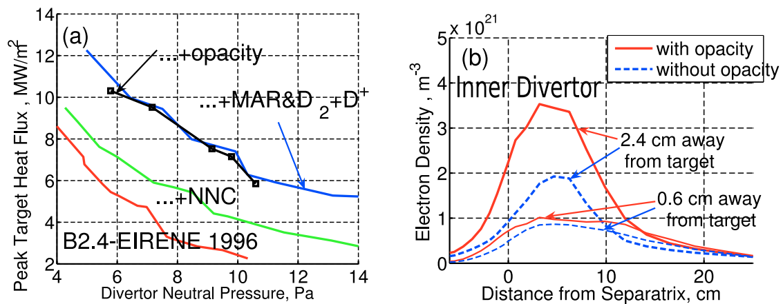
Figure 1: Effect of the new EIRENE for the ITER modelling
