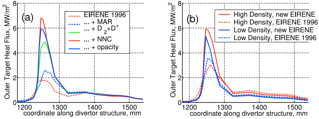
Figure 4: Contributions of the individual effects of the neutral model to the solution
