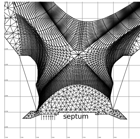
Figure 3: Computational grid and structure for the JET model
