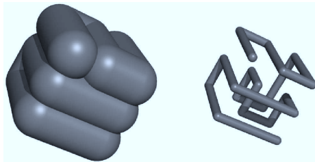
Figure 9: A ground-state conformation for the N = 27 polymer with \rho = 1/\sqrt{2} and r_{ij}^{\text{min}} = 1 (i.e., \sigma \neq 1 ). The left picture shows the conformation in the proper scale, the right side shows the same conformation without proper thickness.
