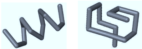
Figure 8: Two N = 13 conformations with \rho = 0.73 ( left ) and \rho = 0.74 ( right ), which are not the ground-state conformations but have a just slightly higher energy than these. The conformations correspond to distinguished ground-state structures at shorter lengths (helical and crystallized on the sc lattice, cp. Fig. 3). For reasons of better visibility, the thickness is not shown on scale.
