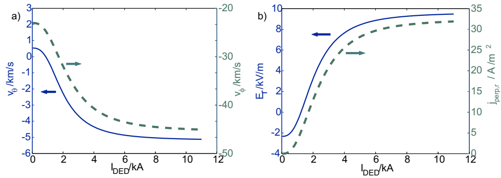
Figure 3: Impact of magnetic perturbation expressed as perturbation current I_{DED} on a) poloidal (solid line) and toroidal rotation (dashed) and b) radial electric field (solid line) and transverse current density (dashed) following as solution from eqns. 1 - 4 (see text for details).
