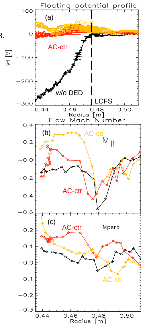
Fig. 4: Profiles of (a) float. pot., (b) paral. and (c) perp. Mach numbers during AC-co and AC-ctr. 3/1 DED.
