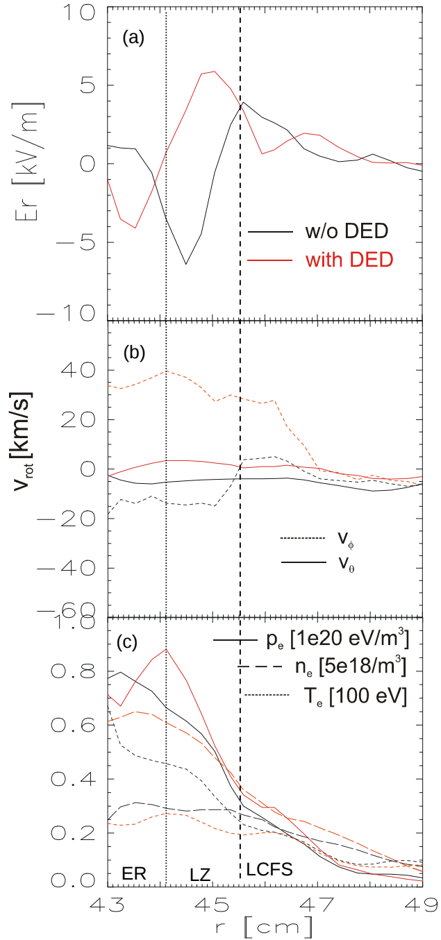
Fig. 2: Profiles of (a) E_r , (b) toroidal v_\phi and poloidal v_\theta rotation and (c) p_e , n_e and T_e , before (black) and during 6/2-DED (red).
