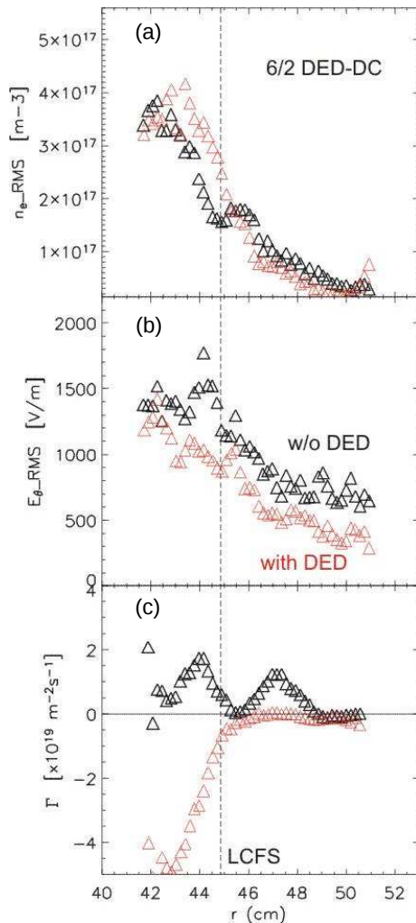
Fig. 3: Profiles of (a) density-, (b) pol. electr. field-fluctuations and (c) turb. part. flux in 6/2 DED.
