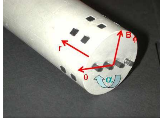
Fig. 1: Mach probe head.
