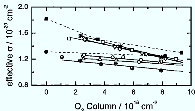
Figure 1. Local effective absorption cross-section \sigma_{\text{O}_2} in the photolysis region vs. \text{O}_2 column between lamp and photolysis region. Open symbols represent the results for our seven Hg-Penray lamps, all operated under same conditions (15mA lamp current, in a slow flow of dry nitrogen). Filled squares and filled circles represent data from Figure 2 (case A and B, respectively) by Lanzendorf et al. for two different Hg lamp operating characteristics.
