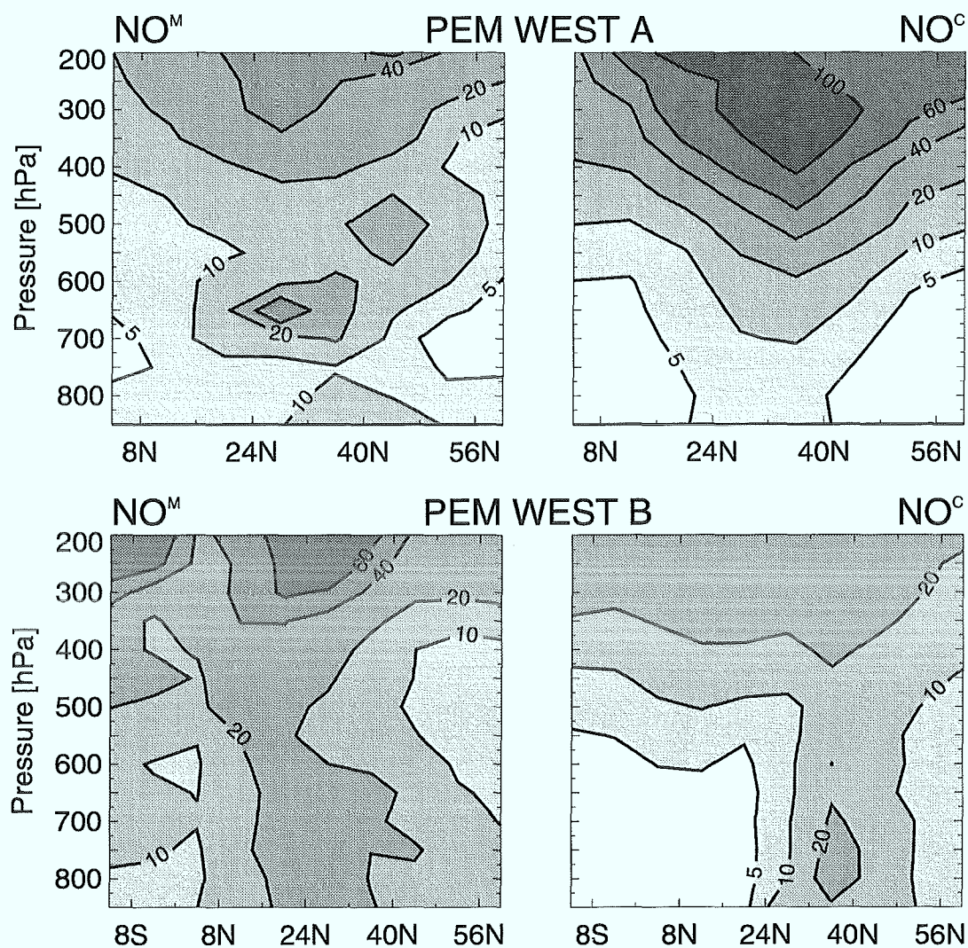
Figure 6.13: Zonally averaged values of the NO mixing ratios (left panels) observed during PEM-West, \mu_{NO}^M , and (right panels) temporal averages \overline{\mu_{NO}^C} calculated along the flight tracks. Upper and lower panels are data for PEM-West A and PEM-West B, respectively.
