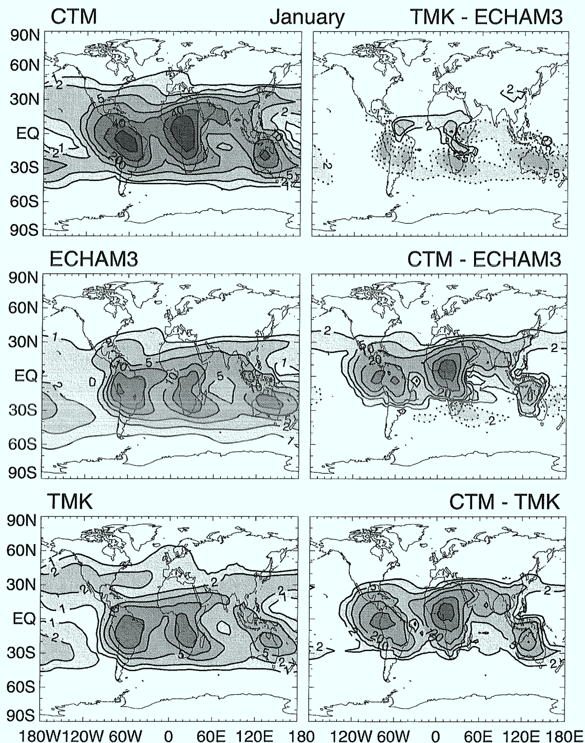
Figure 4.3: Left panels: January monthly mean values of the equivalent ^{222}\text{Rn} concentration, \overline{a_{\text{Rn}}}^m , calculated by the different models at the 200 hPa level. Contours are displayed at 1, 2, 5, 10, 20, 40, and 60 pCi/SCM.
