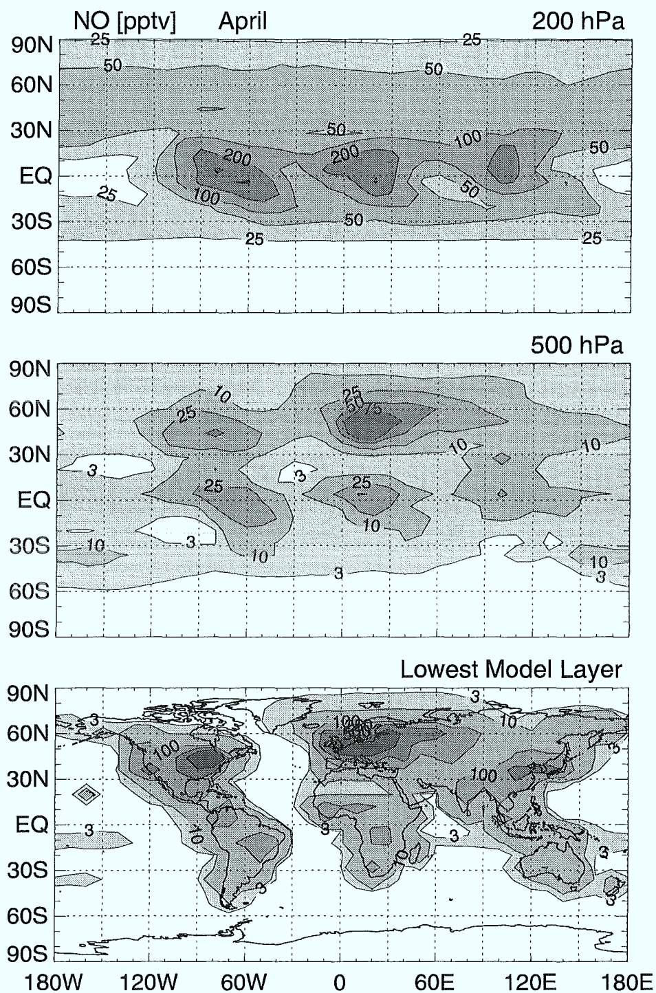
Figure A.2: April monthly mean distributions of NO mixing ratios \overline{\mu_{NO}}^m , calculated with all sources included: (upper panel) 200 hPa level with contours at 25, 50, 100, 200, and 300 pptv, (middle panel) 500 hPa level with contours at 3, 10, 25, 50, and 75 pptv, and (lower panel) the lowest model layer with contours at 3, 10, 100, 250, and 500 pptv.
