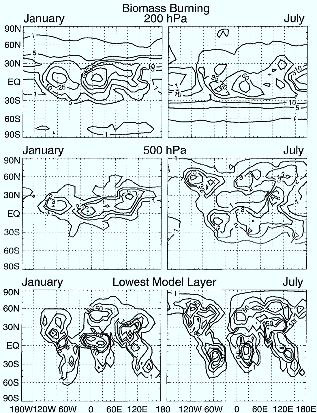
Figure B.4: January and July monthly mean values of \text{NO}_x mixing ratios calculated for the source biomass burning. (Upper panels) 200 hPa level with contours at 1, 5, 10, 25, 50, 100, and 250 pptv, (middle panels) 500 hPa level with contours at 1, 2, 3, 5, and 10 pptv, and (lower panels) the lowest model layer with contours at 1, 10, 50, 100, 250, 500, and 750 pptv.
