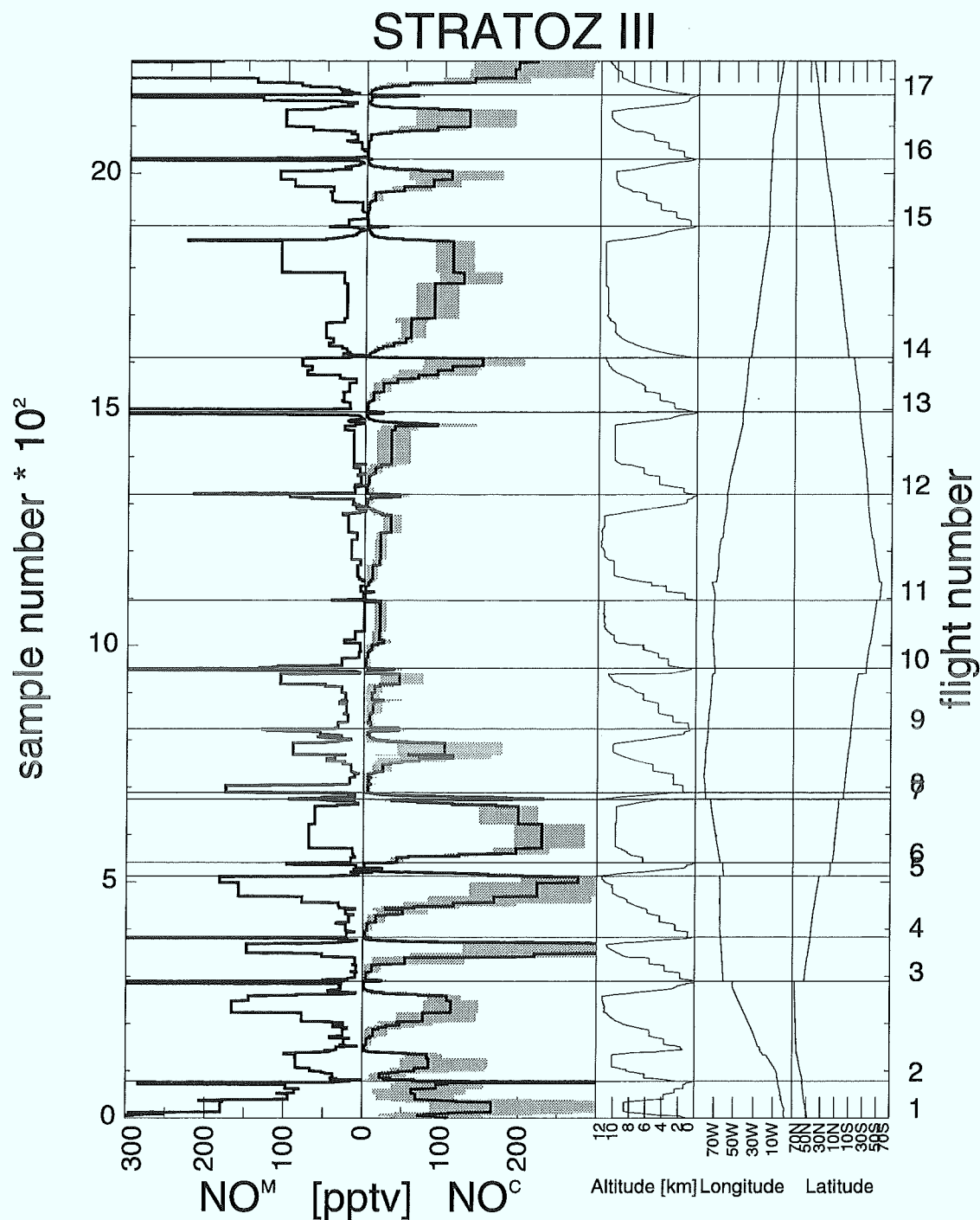
Figure 6.3: Time series of the NO mixing ratios (left part) \mu_{\text{NO}^M} measured during the STRAT0Z III aircraft campaign and (middle part) temporal average \overline{\mu_{\text{NO}^C}^{ca}} calculated along the flight track. The grey shading denotes the range given by the highest and the lowest daily mean value achieved in the CTM during the time period of the campaign. The right part shows the spatial coordinates of the flight tracks.
