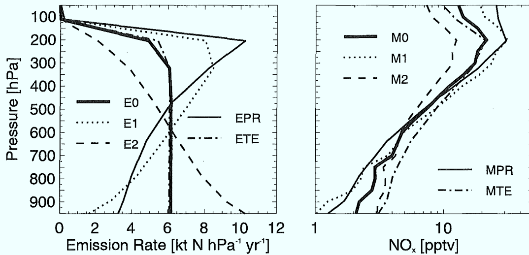
Figure 3.11: Vertical profiles of (left panel) \text{NO}_x emissions and (right panel) the resulting zonally, meridionally, and annually averaged mixing ratios for different CTM runs. The cases 0-2 are based on the standard lightning parametrization (see p. 27), the case PR on the lightning parametrization of Price and Rind [1992], and the case TE on the satellite observations of Turman and Edgar [1982]. See text for details.
