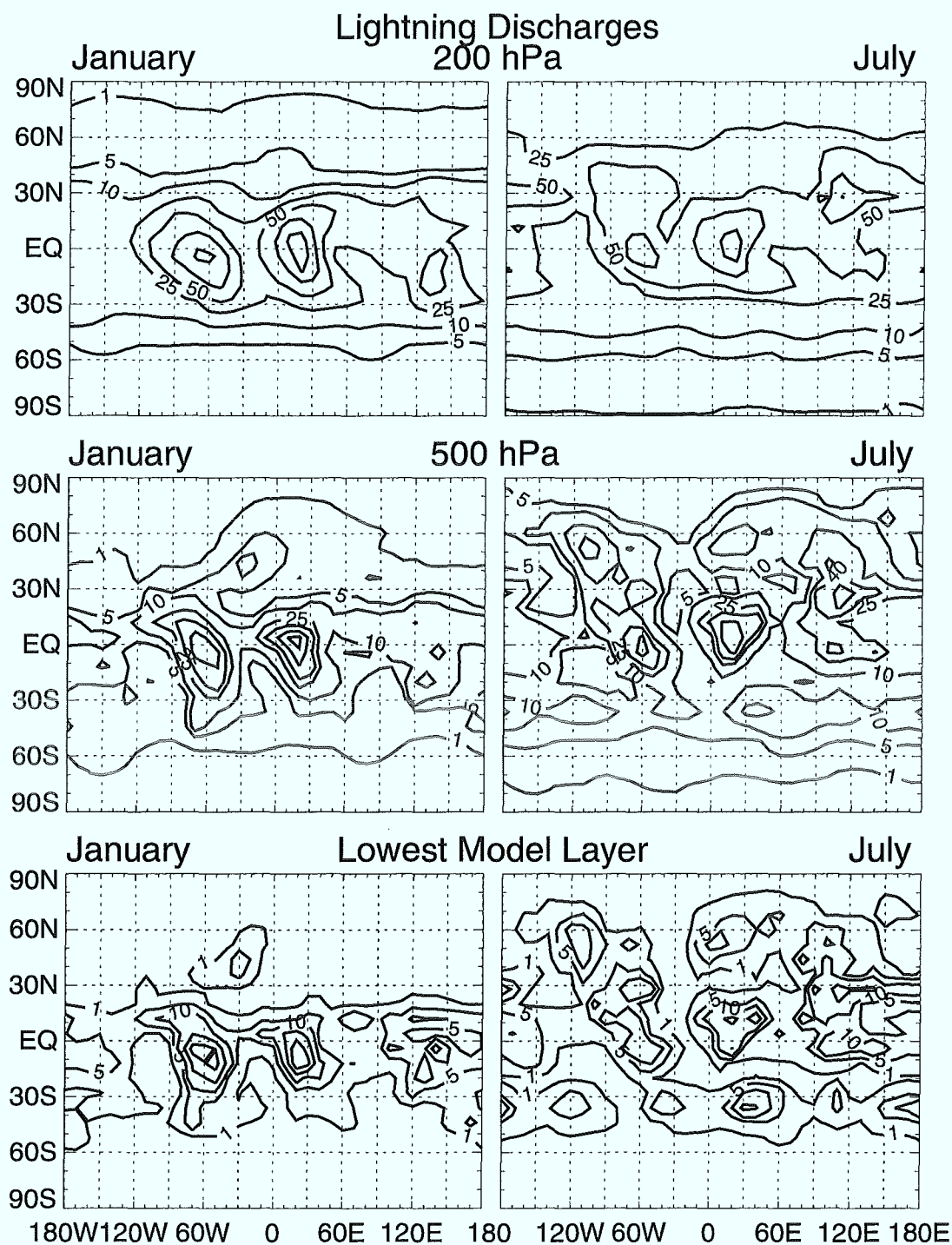
Figure B.3: January and July monthly mean values of \text{NO}_x mixing ratios calculated for the source lightning discharges. (Upper panels) 200 hPa level with contours at 1, 5, 10, 25, 50, 100, and 150 pptv, (middle panels) 500 hPa level with contours at 1, 5, 10, 25, 40, 60, and 80 pptv, and (lower panels) the lowest model layer with contours at 1, 5, 10, 20, and 30 pptv.
