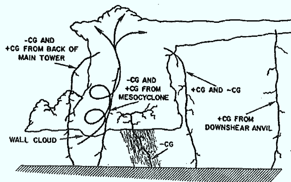
Figure 3.1: Sketch of observed locations of CG flashes from severe thunderstorms. The horizontal scale of this storm sketch is greatly compressed [adopted from Rust et al. , 1981].
