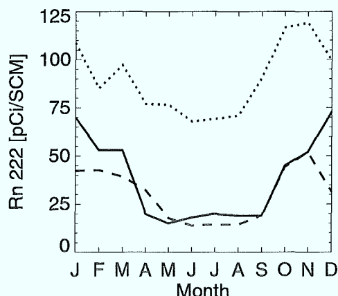
Figure 4.1: Monthly mean equivalent ^{222}\text{Rn} concentrations, \overline{a_{\text{Rn}}}^m , calculated by the CTM for the grid boxes centered at (dotted line) 20^\circ\text{N} , 70^\circ\text{E} and (dashed line) 12^\circ\text{N} , 70^\circ\text{E} as well as (solid line) corresponding observations at Bombay, India 18^\circ\text{N} , 73^\circ\text{E} [Gesell, 1983].
