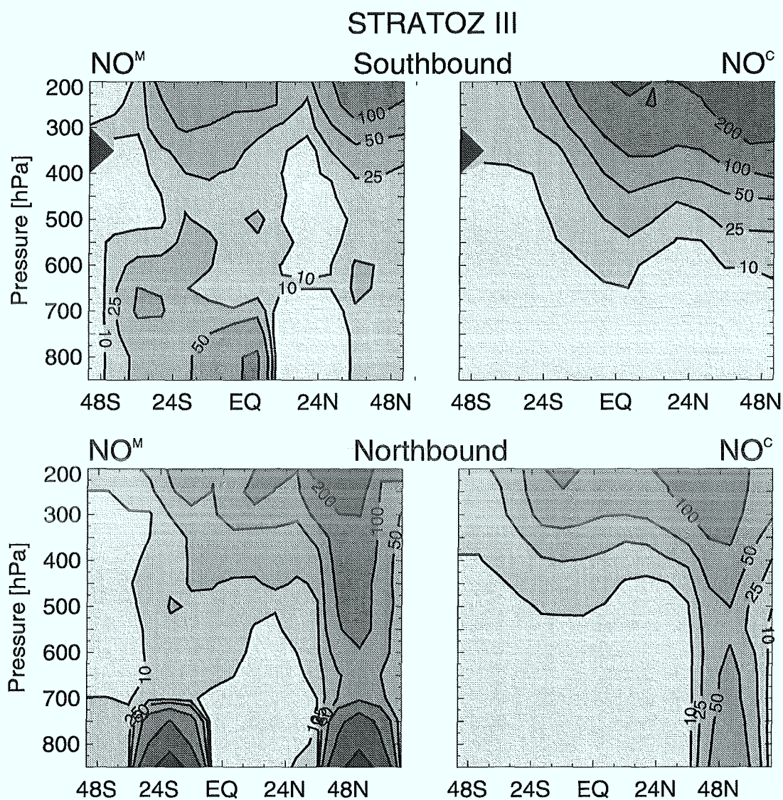
Figure 6.11: Zonally averaged values of the NO mixing ratios (left panels) observed during STRATTOZ III, \mu_{\text{NO}^M} , and (right panels) temporal averages \overline{\mu_{\text{NO}^C}^{ca}} calculated along the flight track. Data from the southbound and northbound flights are averaged separately in the upper and lower panels, respectively.
