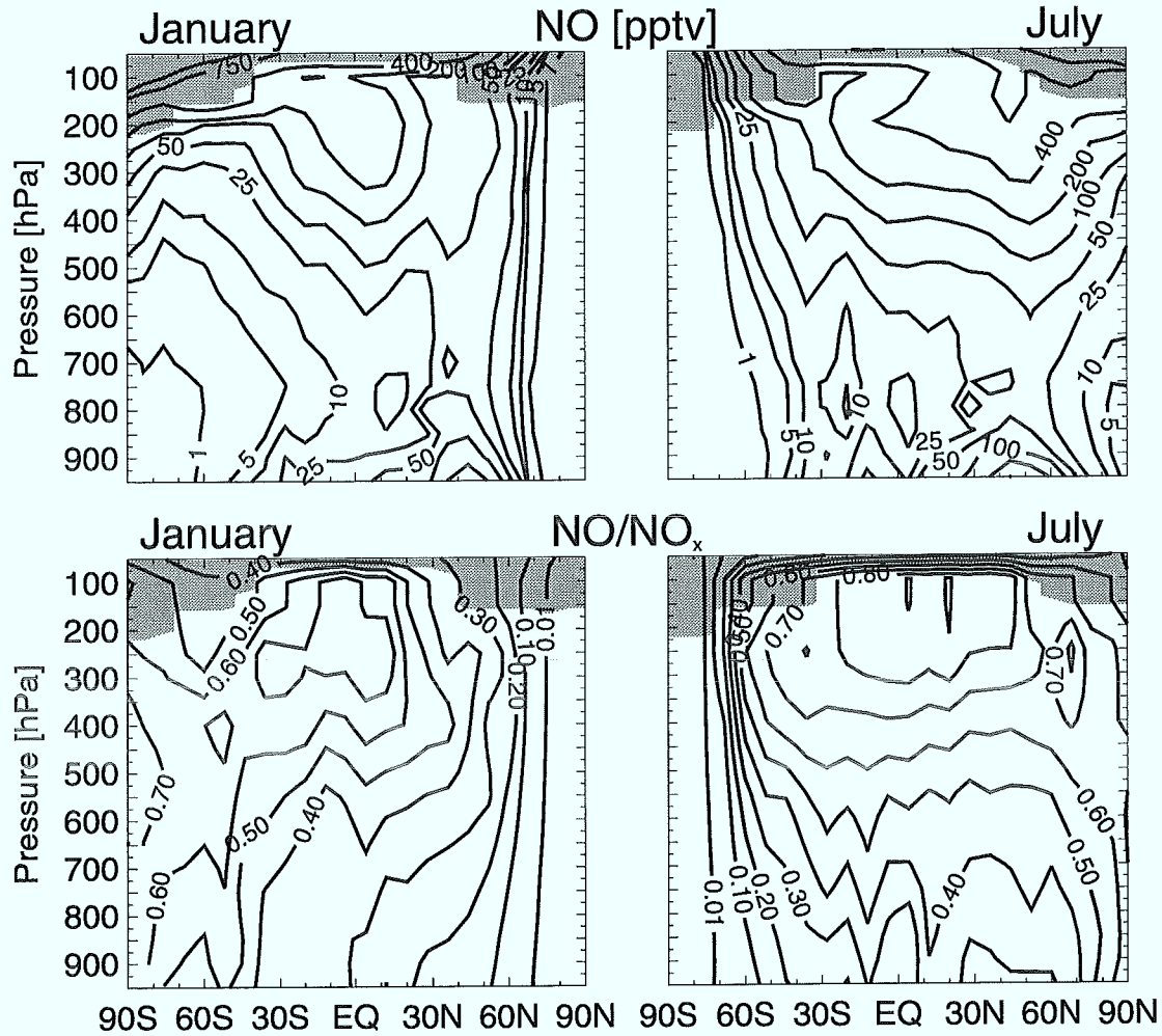
Figure 5.6: Upper panels: Zonal and monthly mean NO mixing ratio, \langle \overline{\text{NO}}^m \rangle_\lambda , calculated with all sources included and contours at 1, 5, 10, 25, 50, 100, 200, 400, 750, and 1000 pptv.
