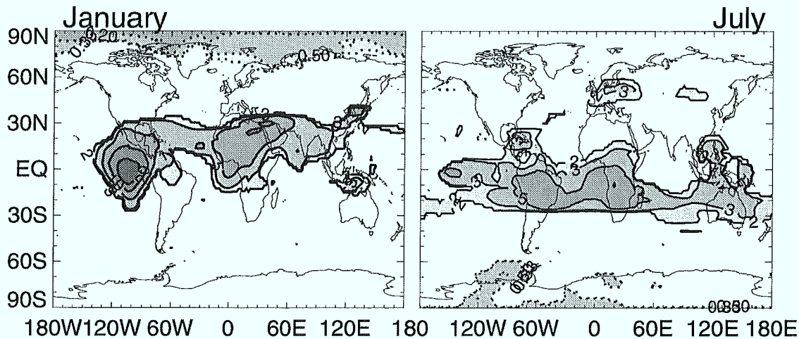
Figure 4.5: Ratio r_{\text{Rn}} = \overline{a_{\text{Rn}}^m} / 0.5(\overline{a_{\text{Rn}}^m} + \overline{a_{\text{Rn}}^m}) at the 200 hPa level. Only those regions are shaded grey, where both \overline{a_{\text{Rn}}^m} and \overline{a_{\text{Rn}}^m} separately differ from \overline{a_{\text{Rn}}^m} by more than a factor of 2. Solid contours are given at 2, 3, 5, 10, and 20, negative ones at 0.2, 0.333, and 0.5.
