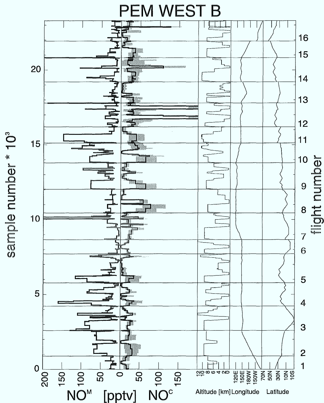
Figure 6.6: Time series of the NO mixing ratios (left part) \mu_{\text{NO}^M} measured during the PEM-West B aircraft campaign and (middle part) temporal average \mu_{\text{NO}^C}^{ca} calculated along the flight track. The grey shading denotes the range given by the highest and the lowest daily mean value achieved in the CTM during the time period of the campaign. The right part shows the spatial coordinates of the flight tracks.
