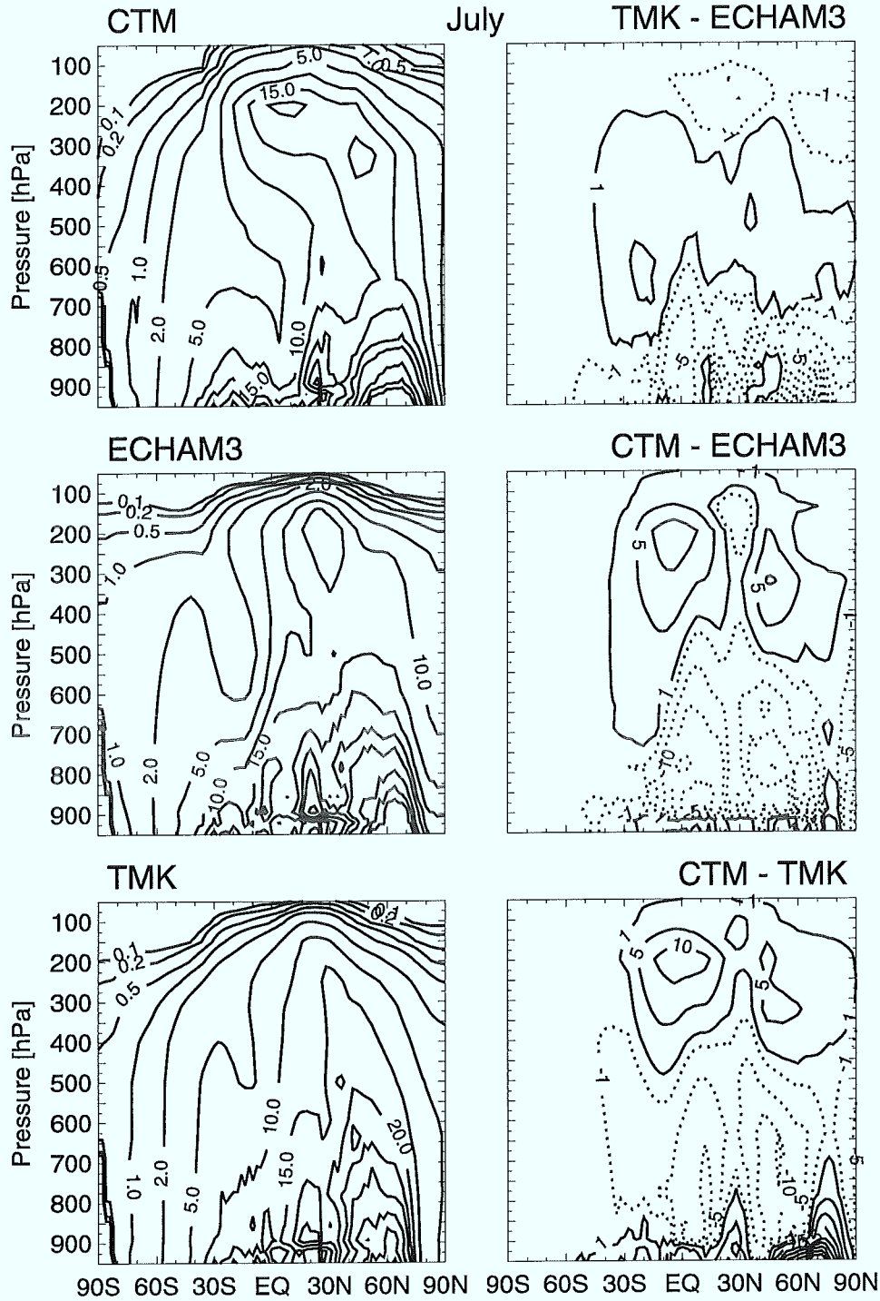
Figure 4.7: Left panels: July monthly mean values of the zonally averaged ^{222}\text{Rn} concentrations, \langle \bar{a}_{\text{Rn}}^m \rangle_\lambda , calculated by the different models. Contours are displayed at 0.1, 0.2, 0.5, 1, 2, 5, 10, 15, 20, 25, 30, 40, 50, and 60 pCi/SCM.
