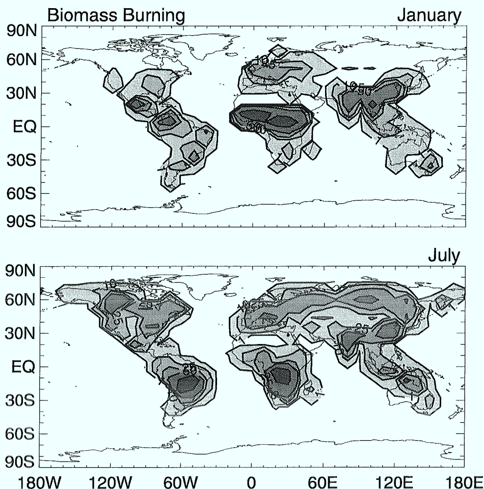
Figure 2.3: Monthly mean NO x emission rates of biomass burning for (upper panel) January and (lower panel) July. Contours are displayed at 1, 10, 25, 50, and 150 mg N m -2 yr -1 .
