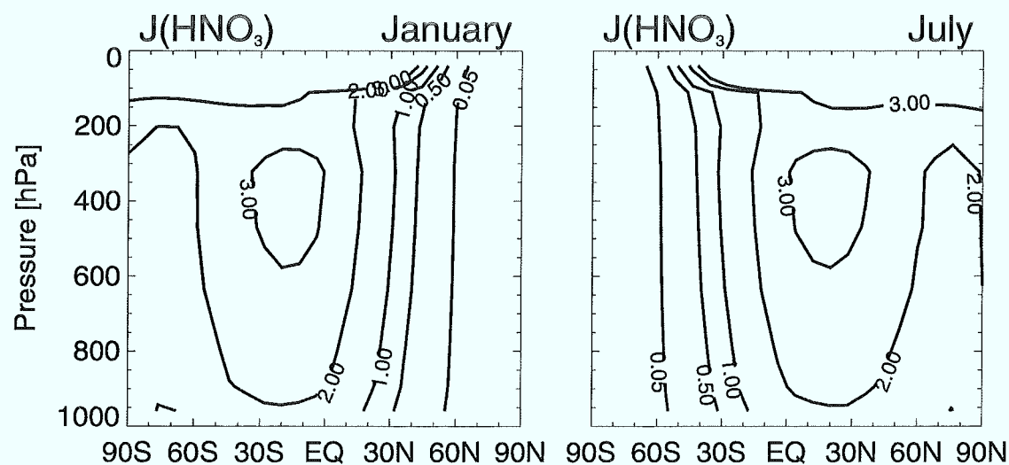
Figure 2.11: Monthly mean values of the photolysis frequency J_{\text{HNO}_3} for (left panel) January and (right panel) July. Contours are displayed at 5 \times 10^{-9} , 5 \times 10^{-8} , 1 \times 10^{-7} , 2 \times 10^{-7} , and 3 \times 10^{-7} \text{ s}^{-1} .
