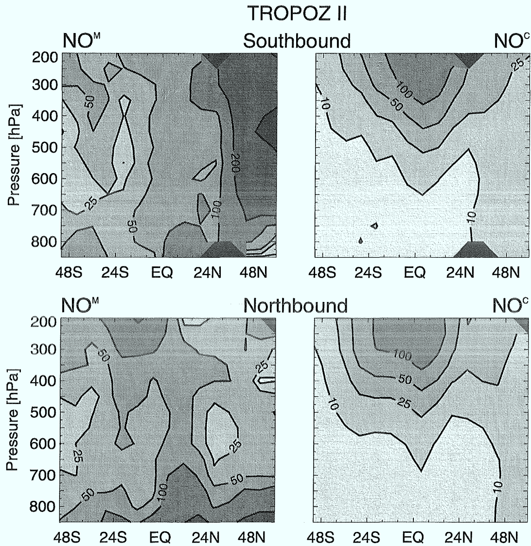
Figure 6.12: Zonally averaged values of the NO mixing ratios (left panels) observed during TROPOZ II \mu_{\text{NO}}^{\text{M}} , and (right panels) temporal averages \mu_{\text{NO}}^{\text{C}a} calculated along the flight track. Data from the southbound and northbound flights are averaged separately in the upper and lower panels, respectively.
