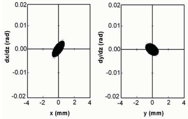
FIG. 9. Phase portrait in front of deflector.
