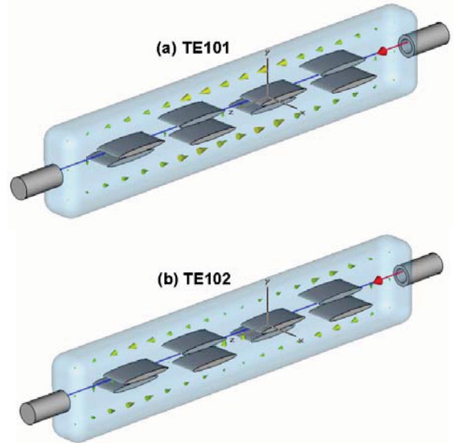
FIG. 13. (Color) TE 101 (a) and TE 102 (b) modes in the rf deflector for f = 1200 MHz.
