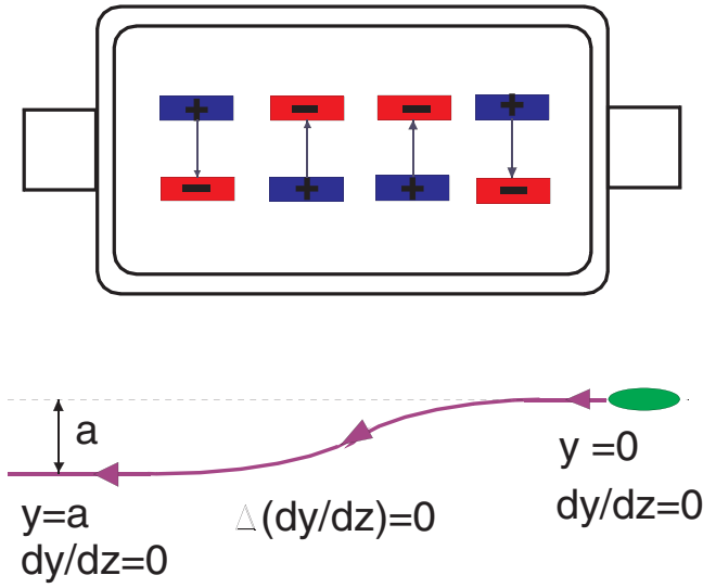
FIG. 11. (Color) The rf deflector with inversion.
