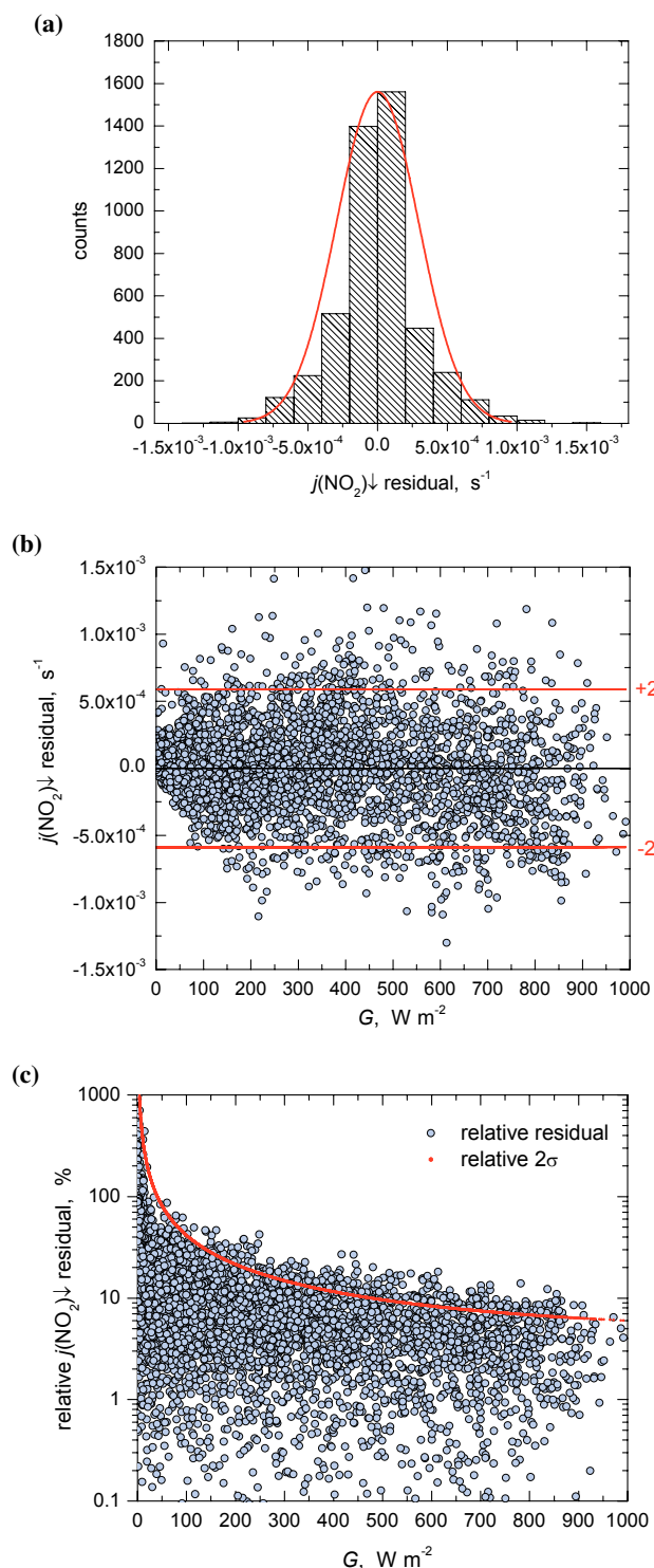
Fig. 3. Residual analysis for polynomial fit shown in Fig. 2b including (a) histogram of the j(\text{NO}_2)\downarrow residuals with Gaussian probability distribution (red line) (b) plot of absolute j(\text{NO}_2)\downarrow residuals versus G with \pm 2\sigma confidence bands (red lines) and (c) relative j(\text{NO}_2)\downarrow residual versus G with relative 2\sigma confidence band (red line).
