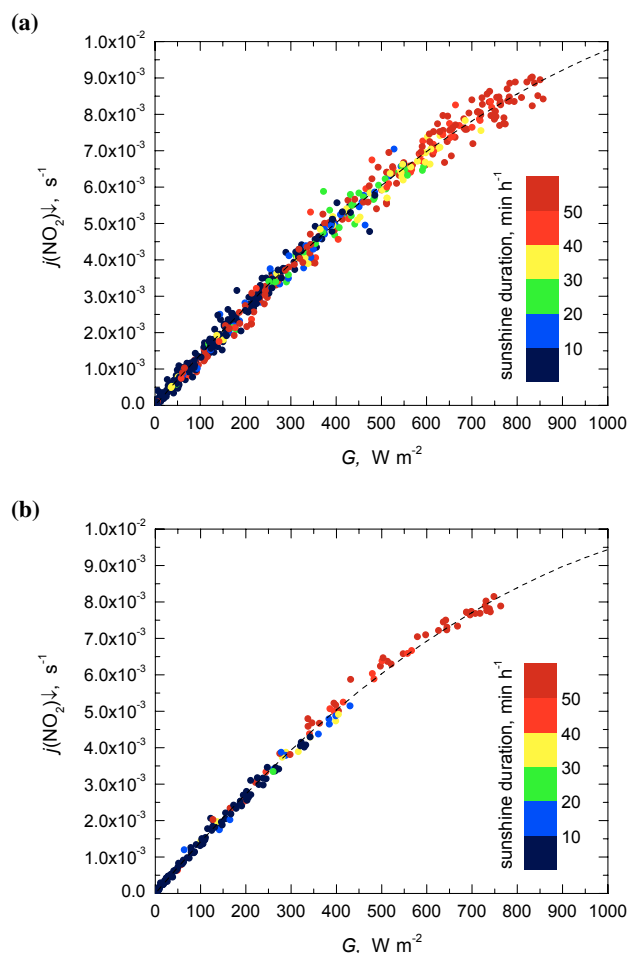
Fig. 6. Scatter plot of j(\text{NO}_2)\downarrow versus G (hourly averages) color-coded with the sunshine duration (0–20 \text{min h}^{-1} : cloudy sky, 20–40 \text{min h}^{-1} : scattered clouds and 40–60 \text{min h}^{-1} : fair weather) for (a) data from Jülich 2002 and (b) data from Hohenpeißenberg 2005. Dashed lines represent the empirical parameterizations for the respective sites from Table 2.
