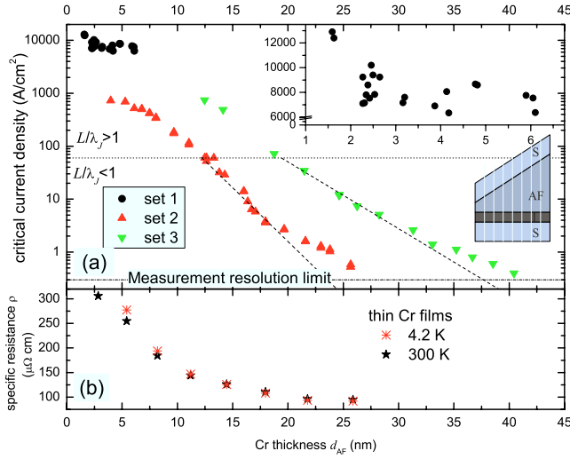
FIG. 3. (Color online) (a) j_c(d_{AF}) of 50 \mu\text{m}^2 (set 1) and 500 \mu\text{m}^2 (sets 2 and 3) JJs and (b) specific resistance \rho of single Cr films. The dotted line indicates the transition from the short to the intermediate JJ length regime. The inset depicts j_c(d_{AF}) of set 1 on a linear scale. Dashed lines are fits to Eq. (4) for short JJs from sets 2 and 3.
