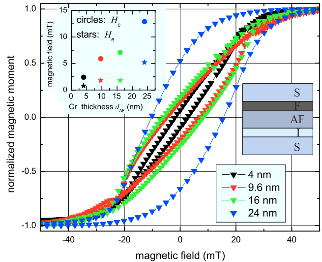
FIG. 4. (Color online) Magnetization of SI-Cr/Fe-S as a function of the in-plane magnetic field for several d_{AF} at 15 K. Exchange bias H_e (stars) and coercivity field H_c (circles) are depicted in the inset. The paramagnetic electrodes tilt the Fe magnetization toward the field axis.
