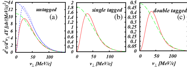
FIG. 2 (color online). The differential cross section d\sigma/d^2v_\perp dY is shown for \rho^0 production at Y = 0 at RHIC (Au-Au collisions with \gamma = 108 ). The solid line is the result including the interference, and the dashed line the result from an incoherent adding of the two processes. The results for the three different tagging cases are given in (a), (b), and (c). The approximate result is shown as a dotted line only in the first (untagged) case. In the other two cases it cannot be distinguished from the full calculation.
