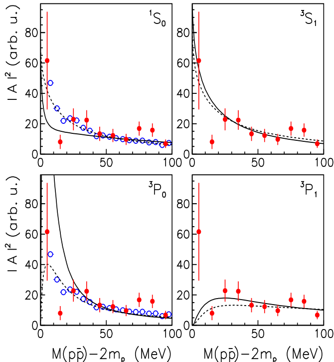
FIG. 1: Invariant B^+ \rightarrow K^+ p\bar{p} amplitude |A|^2 as a function of the p\bar{p} mass. The circles represent the experimental values of |A|^2 extracted from the BaBar data [6] via Eq. (2). The curves are the scattering amplitude squared ( |T|^2 ) predicted by the N\bar{N} model A(OBE) [17] for the ^1S_0 , ^3S_1 , ^3P_0 , and ^3P_1 partial waves and the I=0 (solid) and I=1 (dashed) channels, respectively. Note that the latter results have been normalized to |A|^2 at M(p\bar{p})-2m_p=50 MeV. For comparison reasons we show also the corresponding results extracted from the data on J/\Psi \rightarrow \gamma p\bar{p} [3] (open circles).
